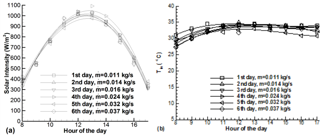
Figure 2: Solar intensity versus time of the day (a), ambient temperatures versus time of the day (b), for different mass flow rates of air at different days.
