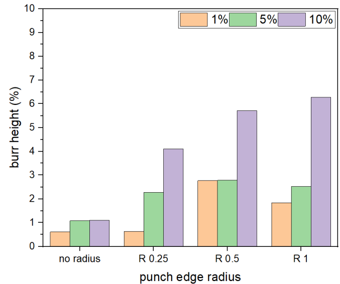
Fig. 5. Burr length - clearance and punch edge radius relation
