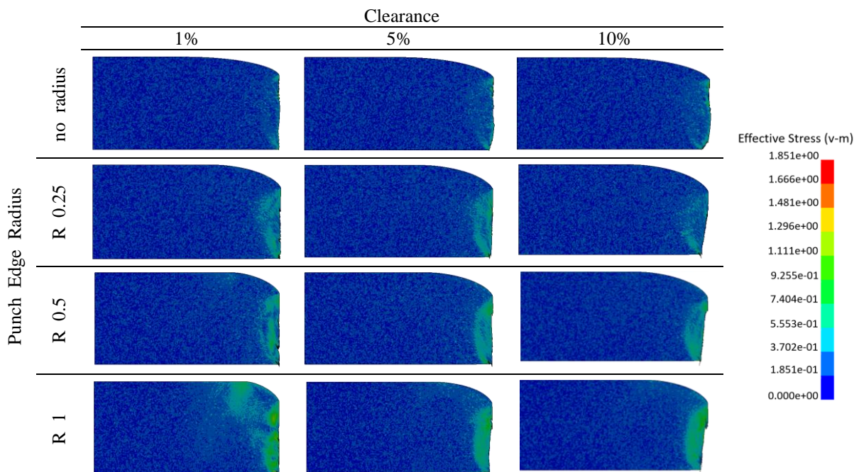
Fig. 10. Stress distributions
