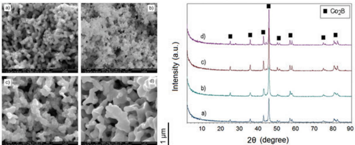
Figure 4. SEM images and X-ray diffraction spectra of cobalt boride particles obtained with different \text{CoCl}_2 initial concentrations. ( \text{CoCl}_2 concentration (mM): (a) 12.6, (b) 25.0, (c) 50.1 (d) 100.1, \text{NaBH}_4/\text{CoCl}_2 molar ratio: 2.4, Reaction time: 12 min, Temperature: +4 °C, Stirring rate: 400 rpm, Ar atmosphere.)
