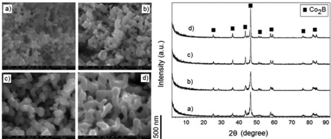
Figure 3. SEM images and X-ray diffraction spectra of cobalt boride particles obtained with different reaction times. (Reaction time (min): (a) 3, (b) 12, (c) 60, (d) 120; \text{CoCl}_2 concentration:25.0 mM; \text{NaBH}_4 concentration:59.50 mM, Temperature: +4 °C; Stirring rate:400 rpm; Ar atmosphere)
