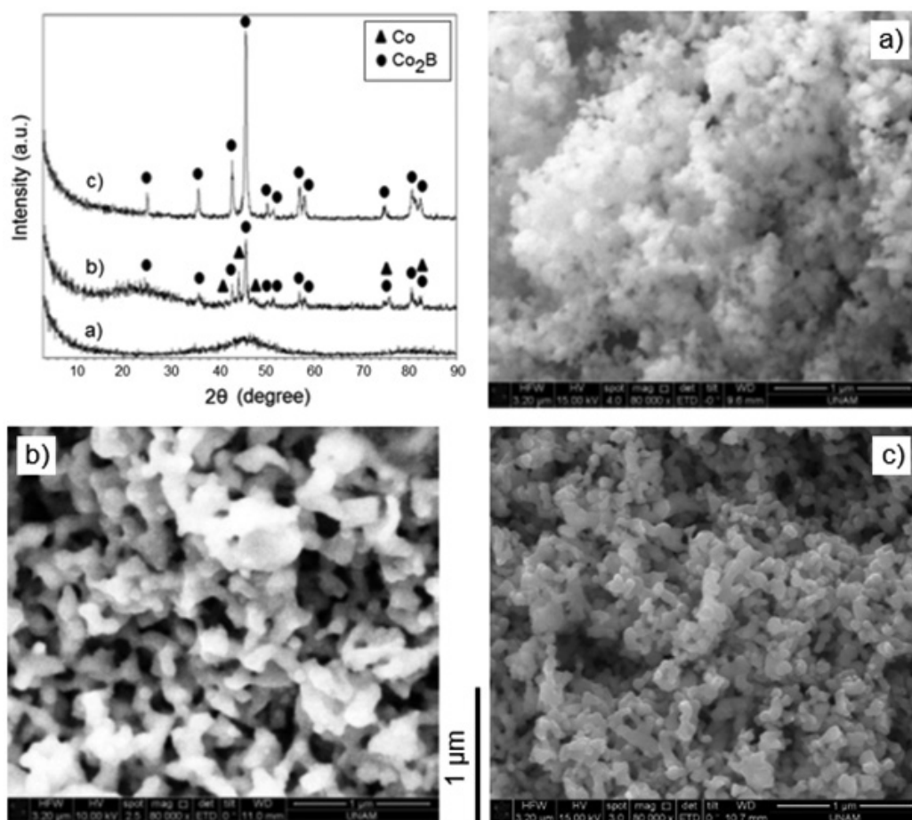
Figure 2. X-Ray diffraction spectra and SEM images of amorphous \text{Co}_2\text{B} (a), crystalline \text{Co-Co}_2\text{B} calcined under air (b), crystalline \text{Co}_2\text{B} calcined under Ar (c).
