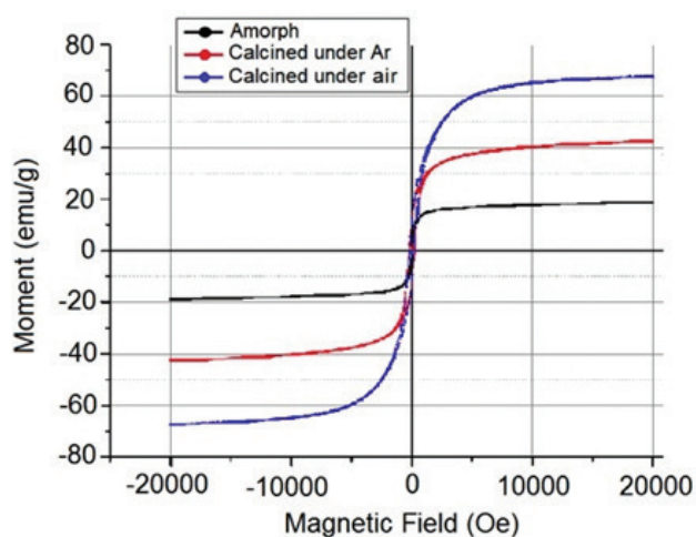
Figure 5. Magnetization curves of the cobalt boride nanoparticles calcined under different conditions
