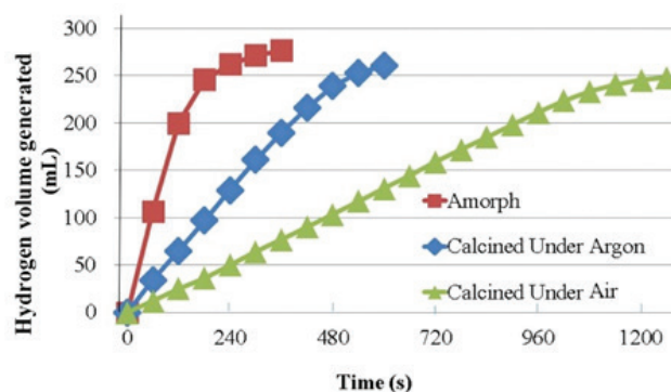
Figure 6. The variation of hydrogen volume with the time by using cobalt boride nanoparticles/nanocylinders obtained with different calcination conditions as catalyst in the hydrolysis of NaBH 4 . (Co 2 B concentration: 10 mg/mL, Initial NaBH 4 concentration: 263.1 mM (~1 % w/w), NaOH concentration: 250 mM, Room temperature).
