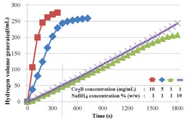
Figure 7. The variation of H 2 volume with the time by using different concentrations of cobalt boride nanoparticles/nanocylinders and different initial NaBH 4 concentrations in the hydrolysis of NaBH 4 . NaOH concentration: 250 mM, Room temperature.
