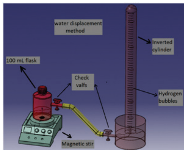
Figure 1. H_2 generation measuring apparatus
