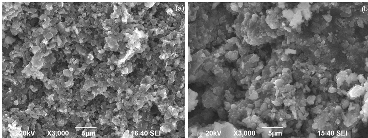
Figure 1. Nominal composition: (a) MgB_2 and (b) Mg_{1.5}B_2 , SEM micrographs
