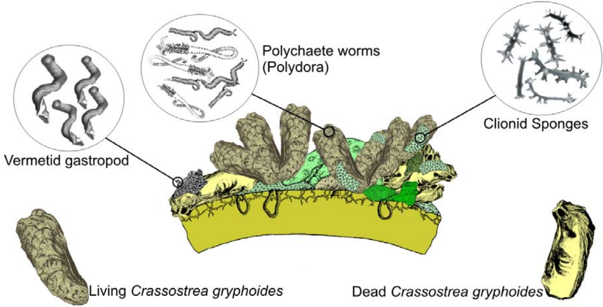
Figure 4. Distribution of a microcommunity structure on a typical heavily encrusted, Early-Middle Miocene Crassostrea gryphoides from K. Maraş. This is the maximum development of endo/epibiont habitation observed on oysters shells from the study area, suggesting a sequence of microcommunities or associations from clionid sponge borings, boring U-shaped polychaete worms and vermetid gastropods.
