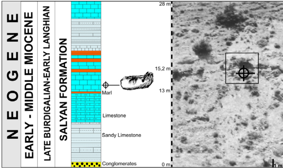
Figure 2. Measured stratigraphic section from Salyan Formation (Hoşgör, 2008).
