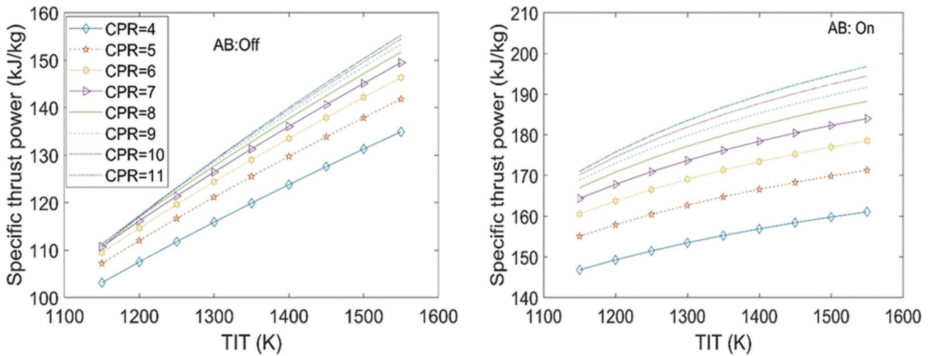
Figure 12. Chngement of STP as a function of CPR and TIT at military and afterburner modes.
