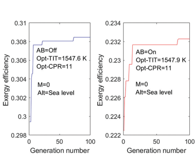
Figure 16. GA optimization of exergy efficiency with TIT and CPR variables at military and afterburner modes.
