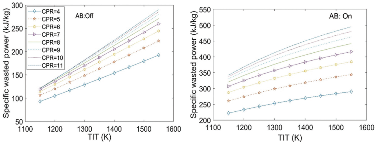
Figure 13. Chngement of SWP as a function of CPR and TIT at military and afterburner modes.
