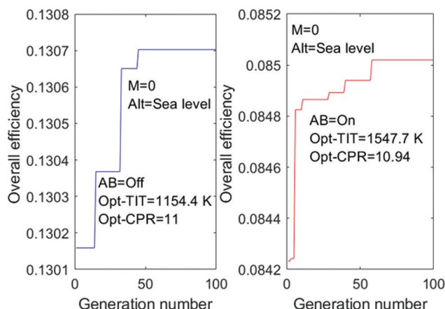
Figure 15. GA optimization of overall efficiency with TIT and CPR variables at military and afterburner modes.
