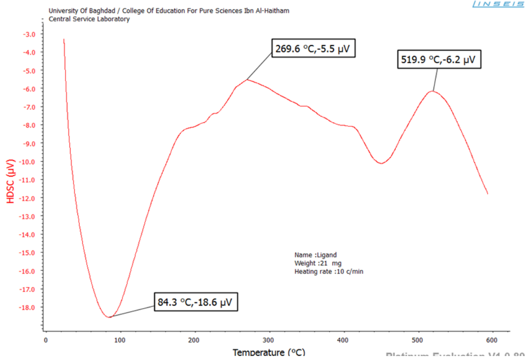
Figure 11: DSC thermogram of an argon atmosphere [L1].
