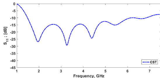
Fig. 2. Return loss plot of the designed DRH antenna
