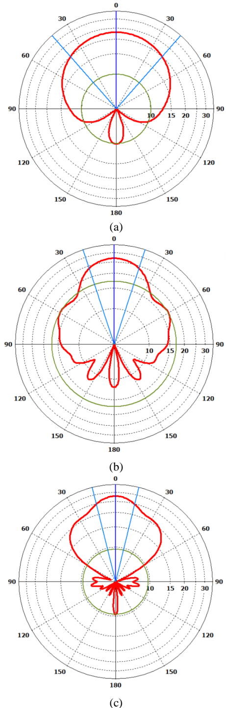
Fig. 3. Azimuth ( \phi ) radiation pattern at elevation angle of \theta=90^\circ for frequencies; (a) 2 GHz, (b) 4.25 GHz and (c) 7 GHz.
