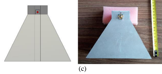
Fig. 4. The designed and produced DRH antenna: (a) perspective view, (b) front view, and (c) top view.
