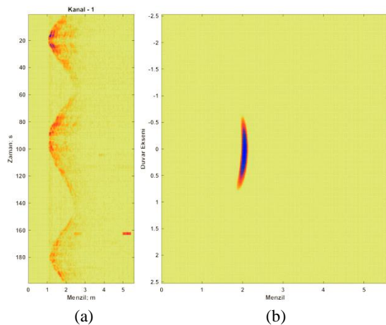
Fig. 7. TWR images obtained by produced DRH antennas: (a) Range-time image, (b) Range-cross range image
