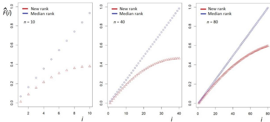
Figure 2. A comparison between values of the new rank estimator and median rank estimator
