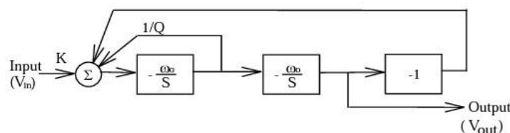
Figure 5. Block diagram of a quadratic filter [38]
