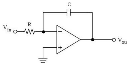
Figure 4. A low-pass filter circuit [38]
