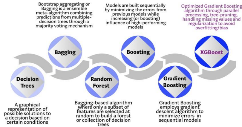
Figure 1: XGBoost Evolution
