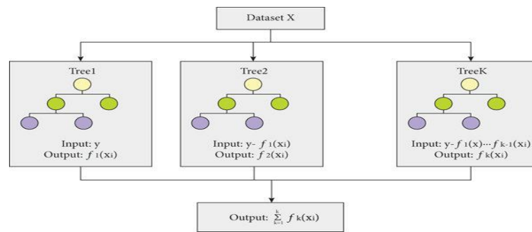
Figure 2: XGBoost Architecture
