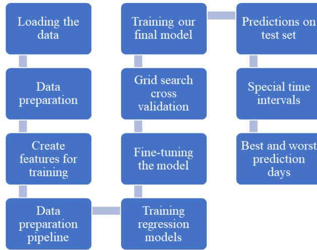
Figure 4. Our methodology
