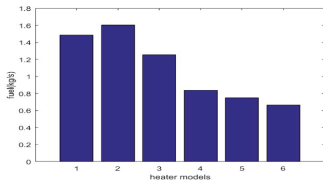
Figure 15. Comparison of fuel consumption in different models.
