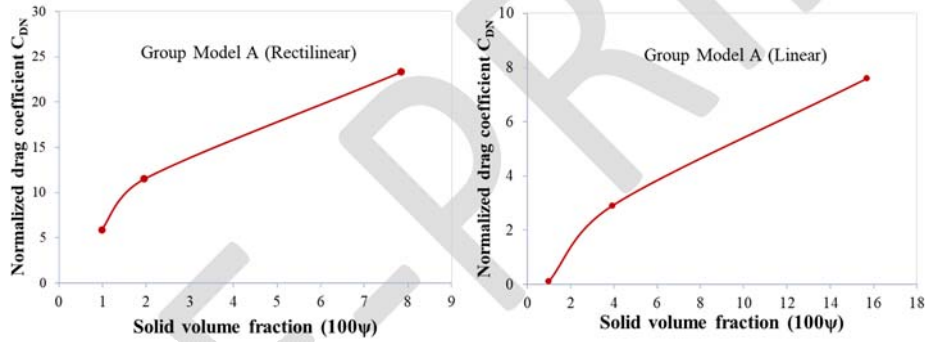
Fig 14 - Variation of C_{DN} with various \psi for group model A (Linear and Rectilinear).
