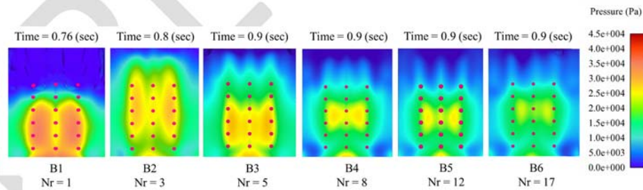
Fig 12 - The Pressure distributions in the 18 measurement points on the rigid wall for group models B with various \phi , (0.04, 0.12, 0.2, 0.31, 0.47 and 0.67).
