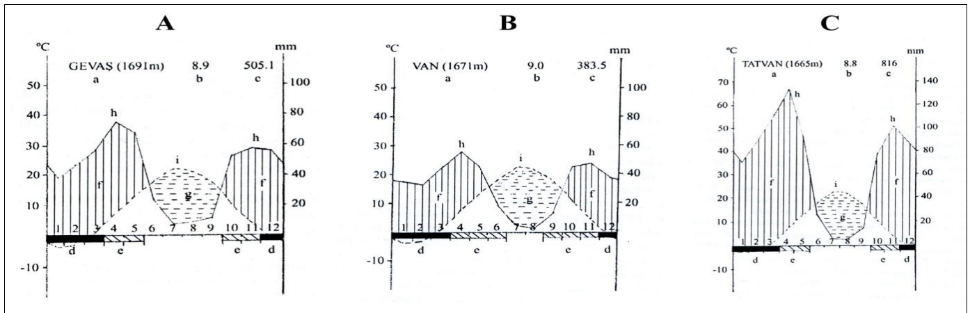
Figure 2. Ombrothermic diagrams of Gevaş (A), Van (B) and Tatvan (C)
