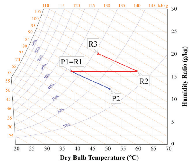
Figure 2. Psychrometric diagram for 60 °C regeneration temperature and 1.3 m/s air frontal velocity.
