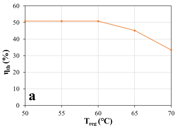
Figure 8. Variation of thermal (a), solar cell and module efficiency (b) with regeneration temperature.
