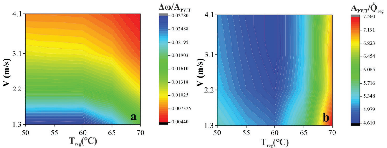
Figure 9. Variation of moisture removed per PV/T area (a) and required PV/T area per regeneration thermal energy (b) with regeneration temperature and air frontal velocity.
