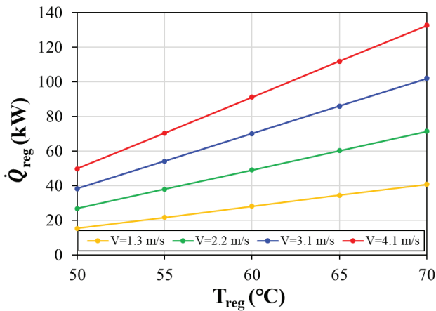
Figure 5. Effect of regeneration temperature on required regeneration thermal energy
