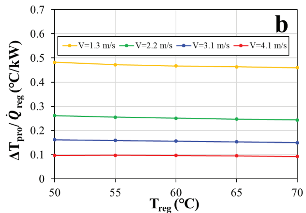
Figure 6. Variation of ( \Delta\omega_{pro}/\dot{Q}_{reg} ) (a) and ( \Delta T_{pro}/\dot{Q}_{reg} ) (b) with regeneration temperature
