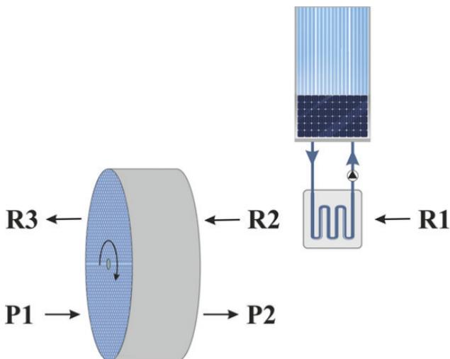
Figure 1. Schematic view of the desiccant wheel studied.
