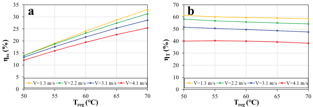
Figure 4. Dehumidification (a) and temperature effectiveness (b) of desiccant wheel.
