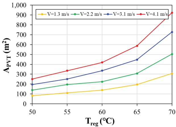
Figure 7. Effect of regeneration temperature on required PV/T collector area.
