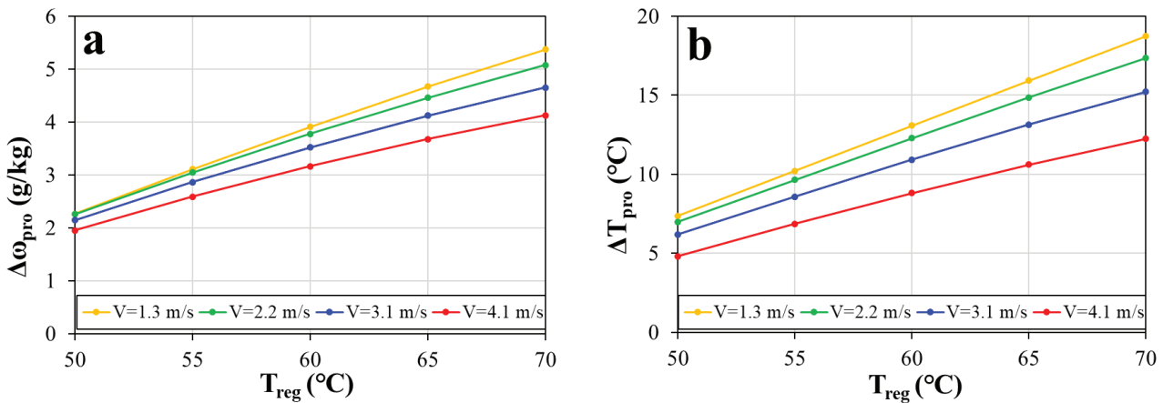
Figure 3. Variation of moisture removed (a) and temperature increase (b) in desiccant wheel with regeneration temperature.
