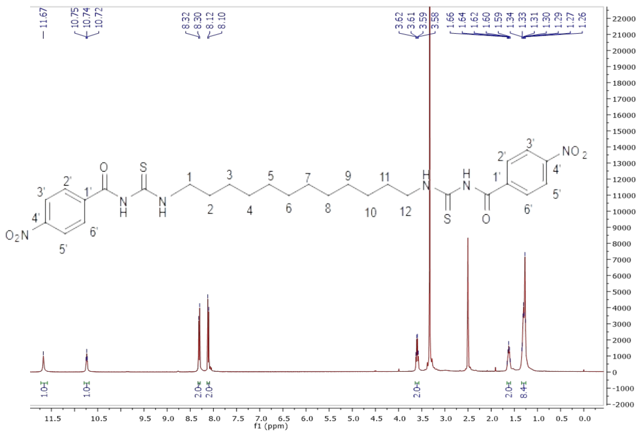
Figure S1. ^1\text{H} NMR spectra of 5
