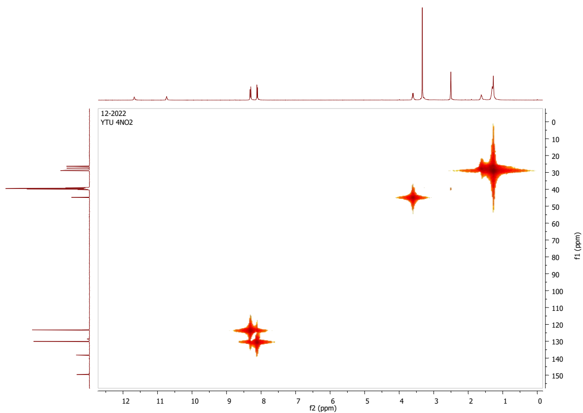
Figure S5. HMQC spectra of 5
