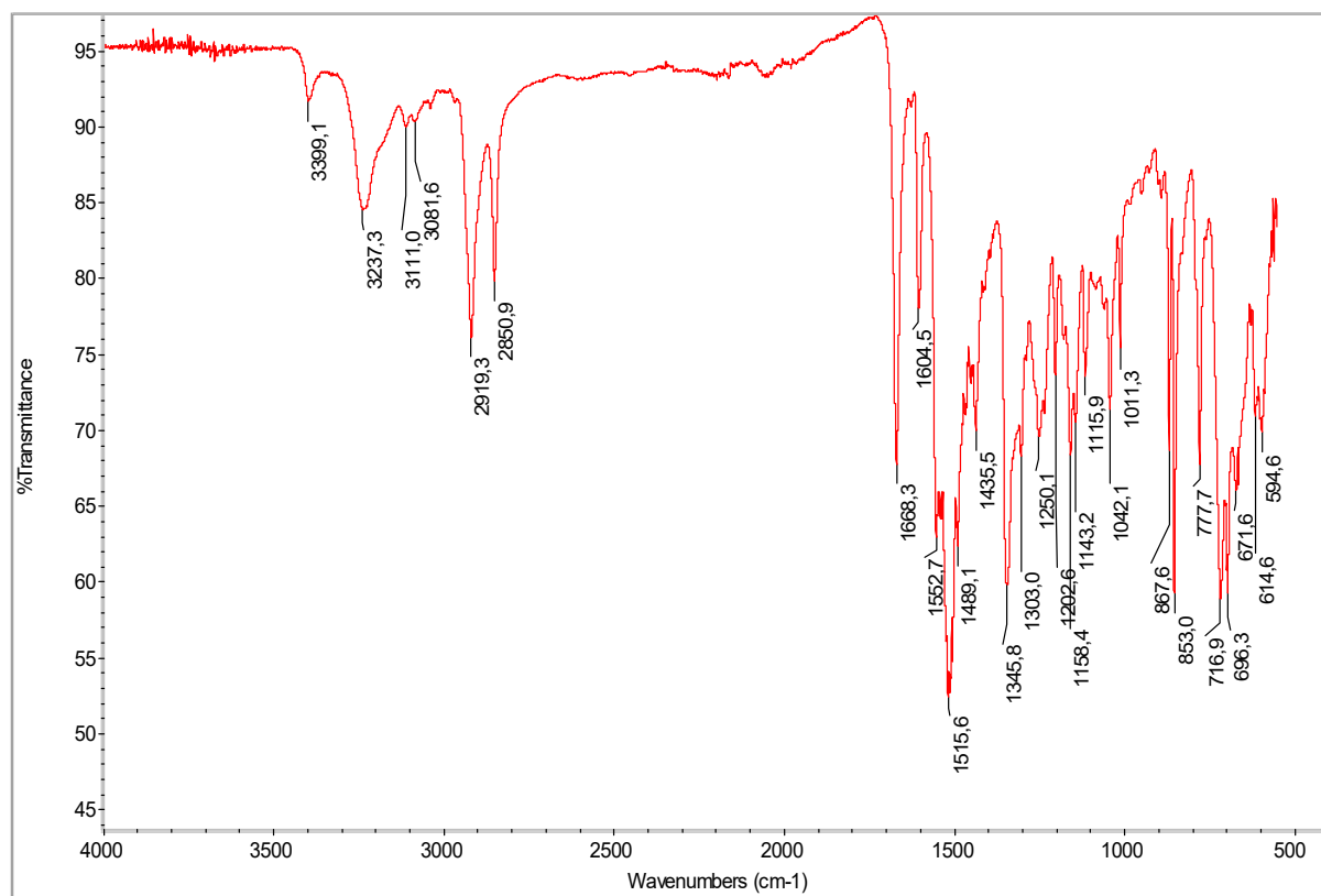
Figure S6. FT-IR spectra of 5
