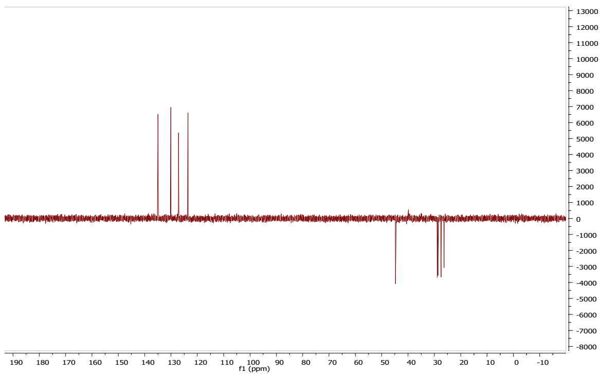
Figure S9. DEPT spectra of 6
