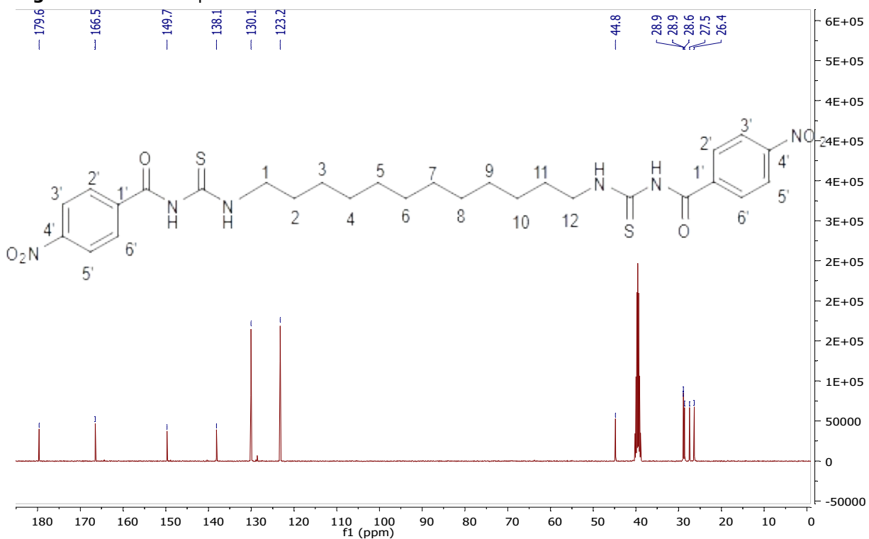
Figure S2. ^{13}\text{C} NMR spectra of 5
