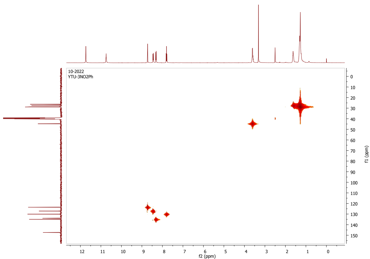
Figure S11. HMQC spectra of 6
