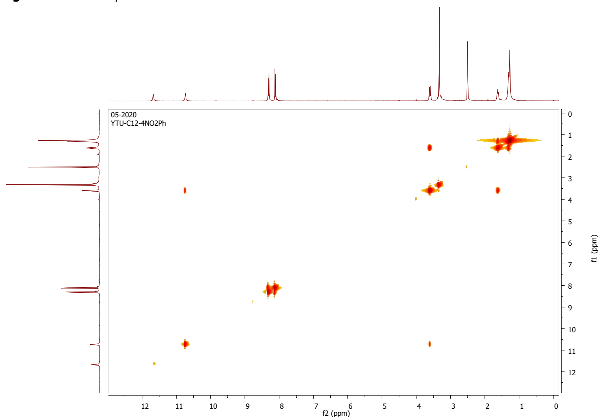
Figure S4. COSY spectra of 5
