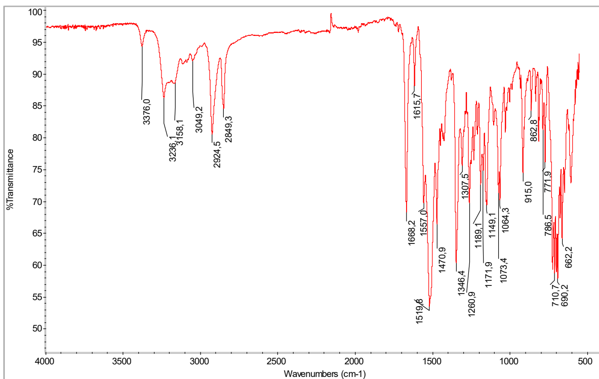
Figure S12. FT-IR spectra of 6
