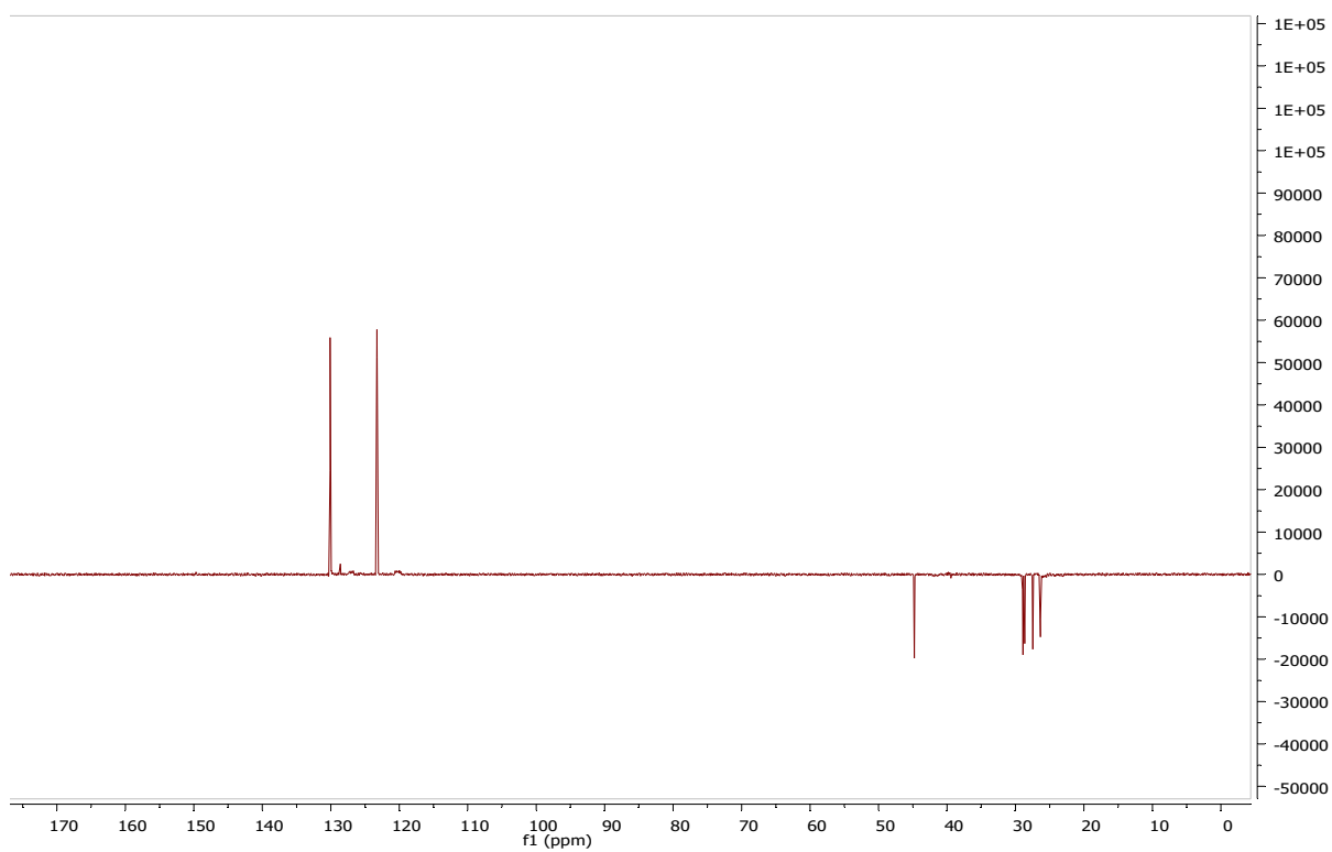
Figure S3. DEPT spectra of 5
