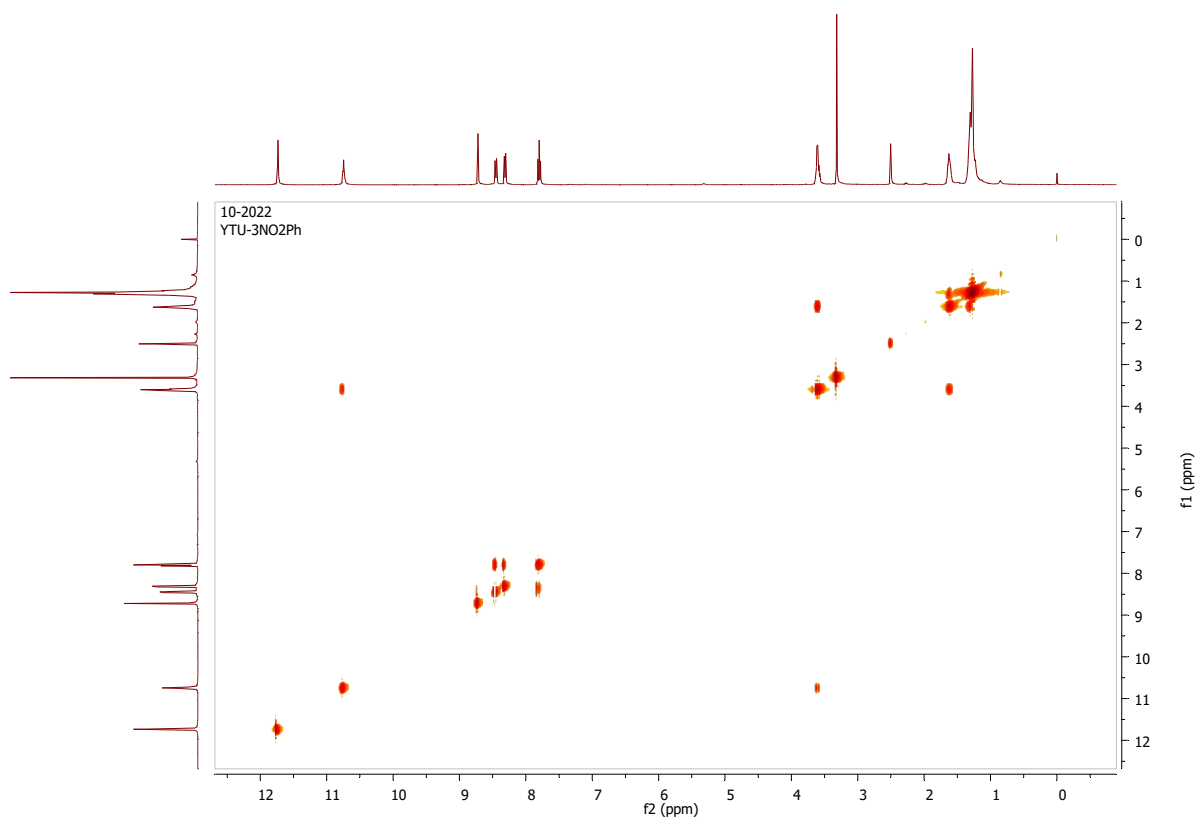
Figure S10. COSY spectra of 6
