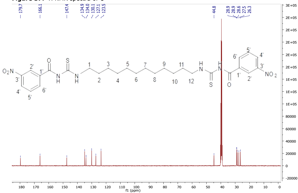
Figure S8. ^{13}\text{C} NMR spectra of 6
