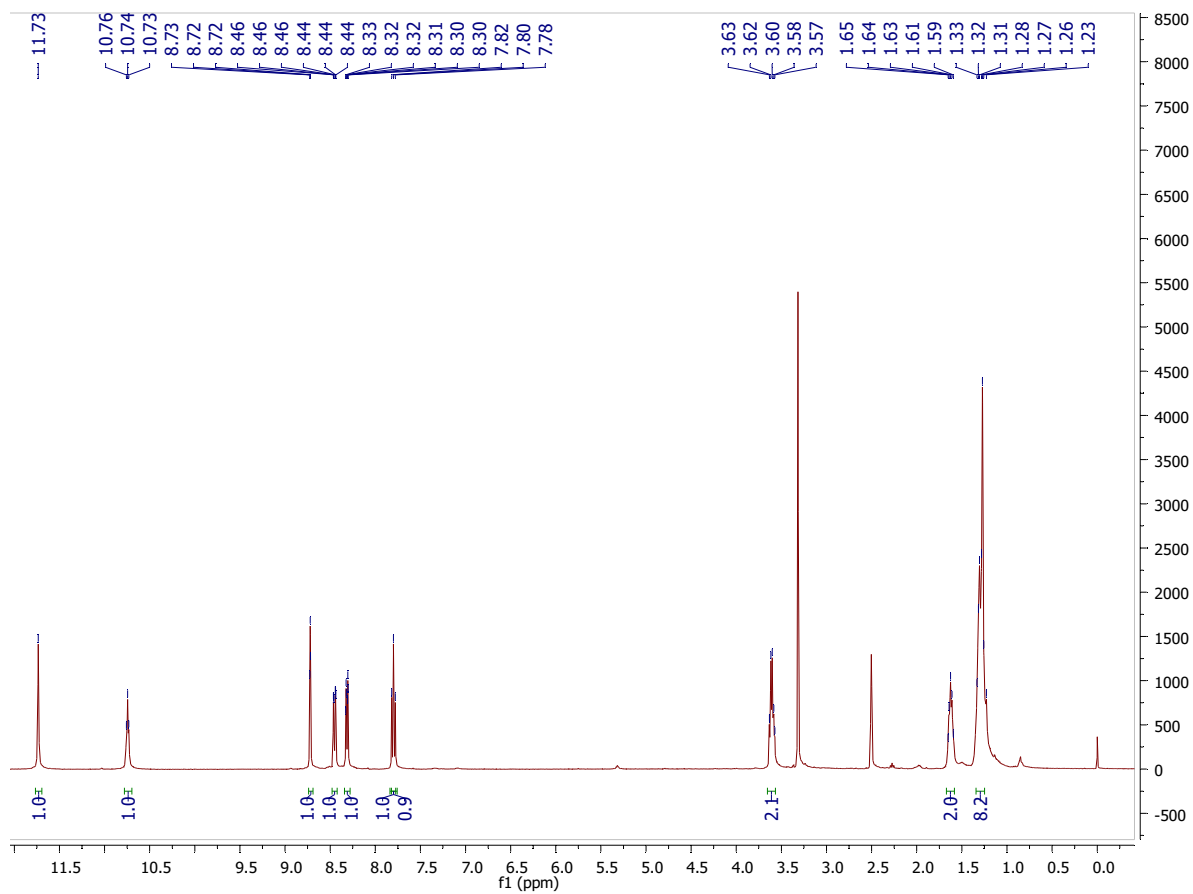
Figure S7. ^1\text{H} NMR spectra of 6
