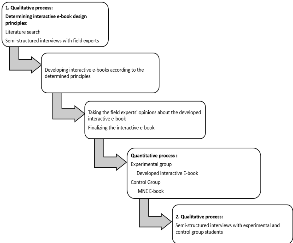
Figure 1. Research Design
