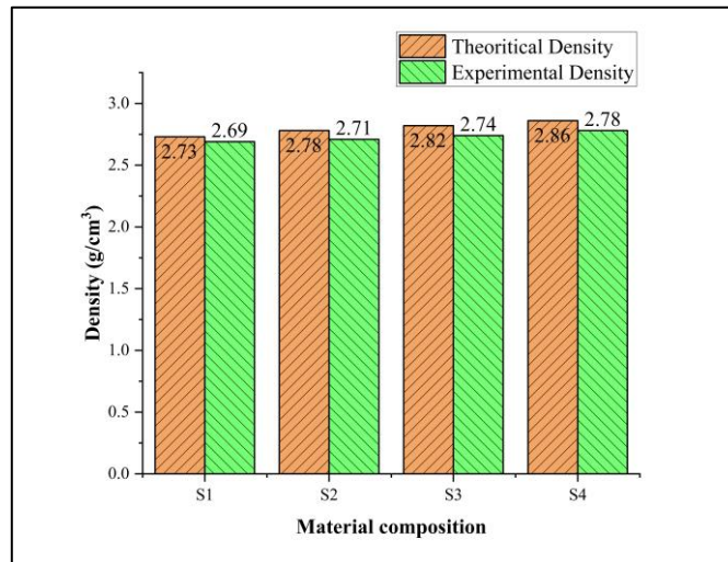
Figure 9. Shows the variations of sintered density with different samples
