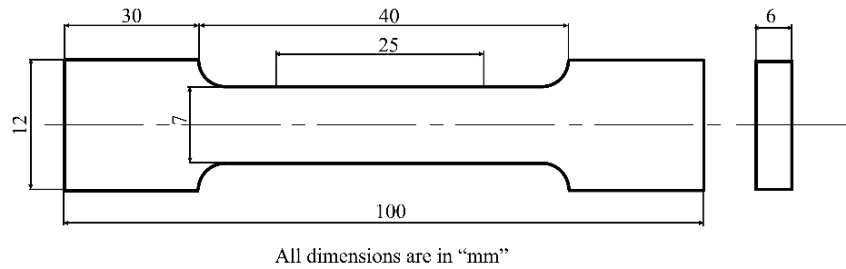
Figure 4. ASTM E-8-04 standard tensile test specimen
