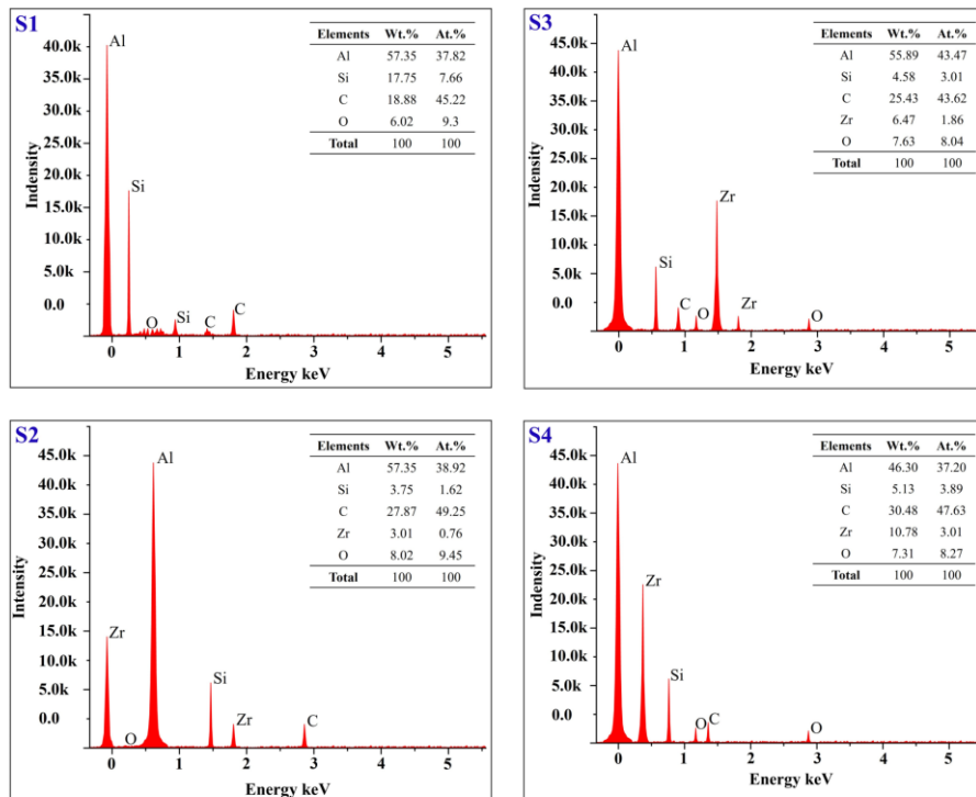
Figure 8. Shows that the energy dispersive X-ray spectroscopy (EDX) analysis result
