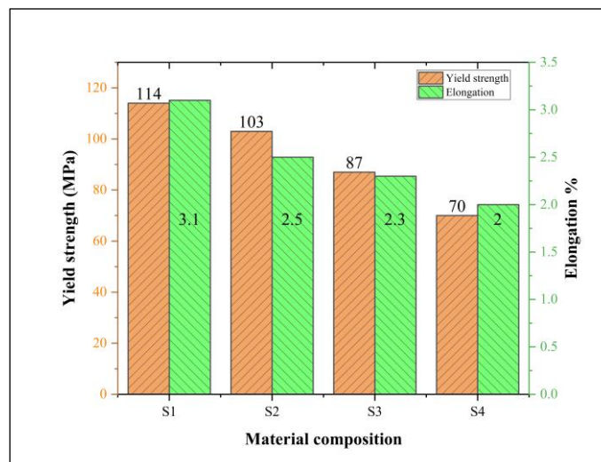
Figure 13. Shows the elongation of the hybrid composite materials
