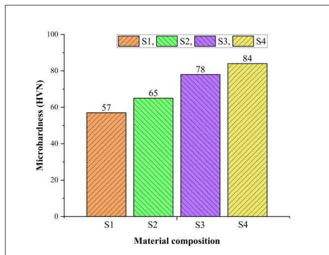
Figure 11. Shows the microhardness of hybrid composite materials
