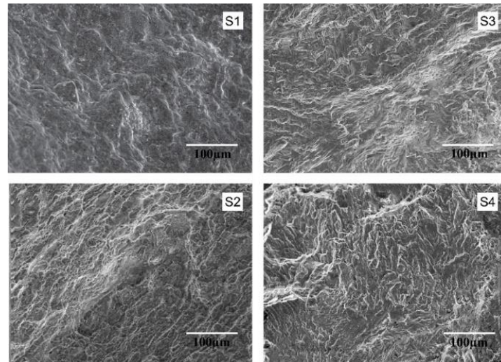
Figure 15. Shows the compressive test fracture
