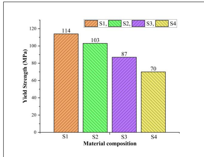
Figure 12. Shows the yield strength of the hybrid composite materials
