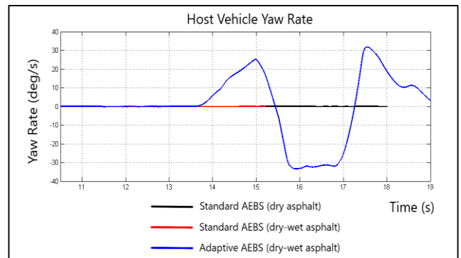
Fig. 9. Host vehicle yaw rate
