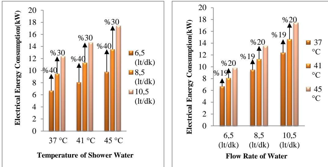
Figure 6. Percentage change in energy consumption of M-2 based on sewage water flow rate and shower water temperature
