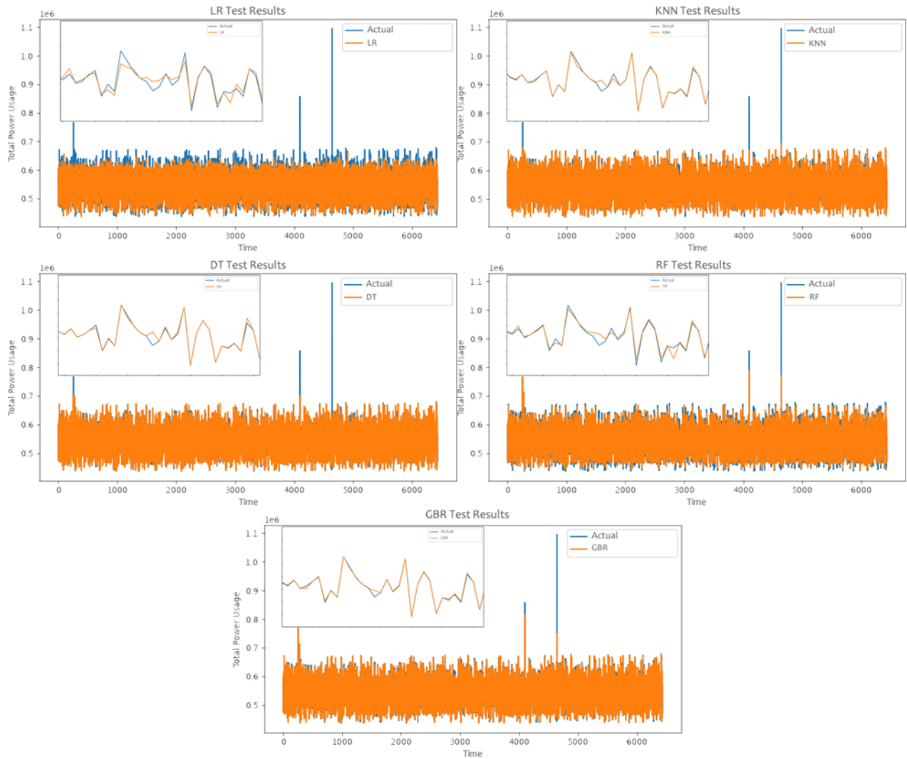
Figure 1. Test results of regression models
