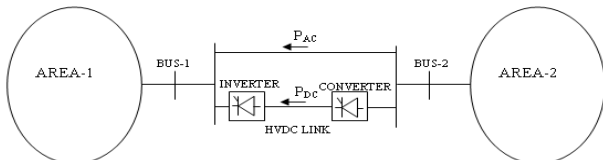
Fig. 1. An HVDC Link in a parallel AC-DC interconnected power system
