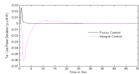
Fig.7. Tie line power deviation (10% Disturbance)
