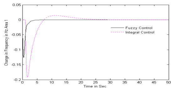
Fig.5. Frequency deviation in area-1(10% Disturbance)
