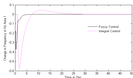
Fig.8. Frequency deviation in area-1(30% Disturbance)
