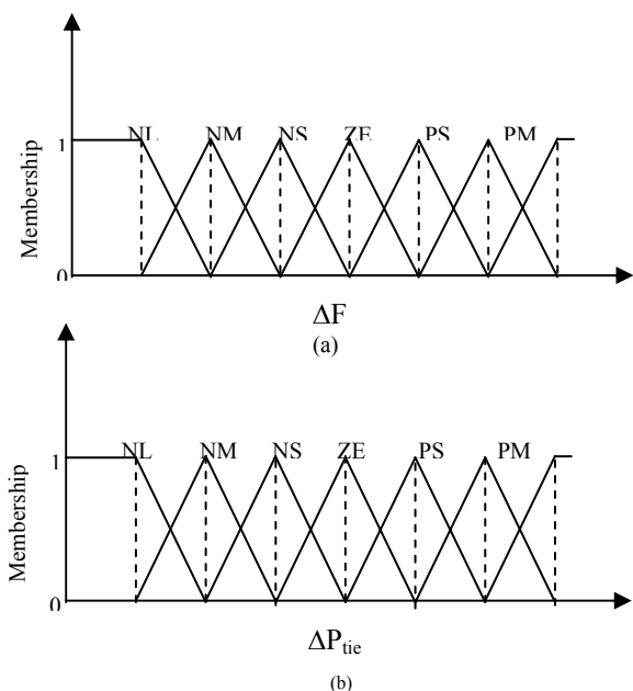
Fig.3. Input membership functions of fuzzy controller (a) \Delta F ; (b) \Delta P_{tie}
