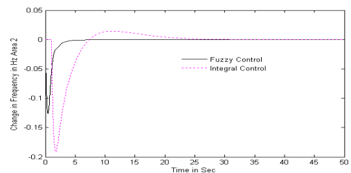
Fig.6. Frequency deviation in area-2(10% Disturbance)
