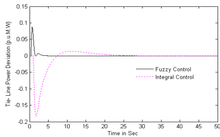
Fig.10. Tie line power deviation (30% Disturbance)
