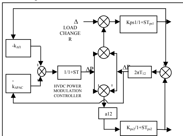
Fig. 2. Linearized Model of Interconnected Power System without Governors for Control Design of Power Modulation Controller of HVDC Link.
