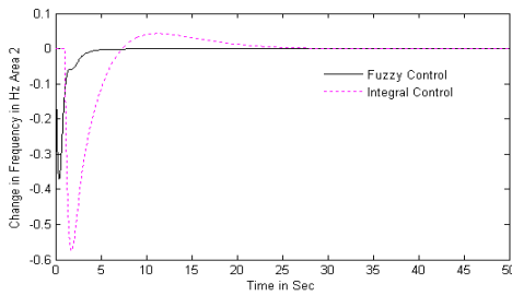
Fig.9. Frequency deviation in area-2(30% Disturbance)
