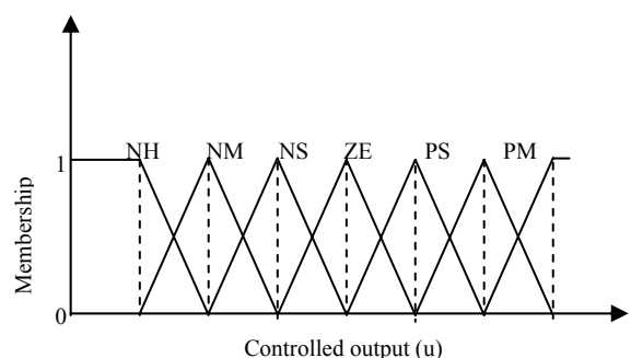
Fig.4 Output membership functions of fuzzy controller
