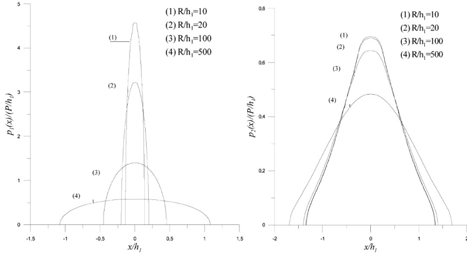
Fig. 5a - Contact stress distribution between circular rigid block and homogeneous layer for various values of R/h_1
