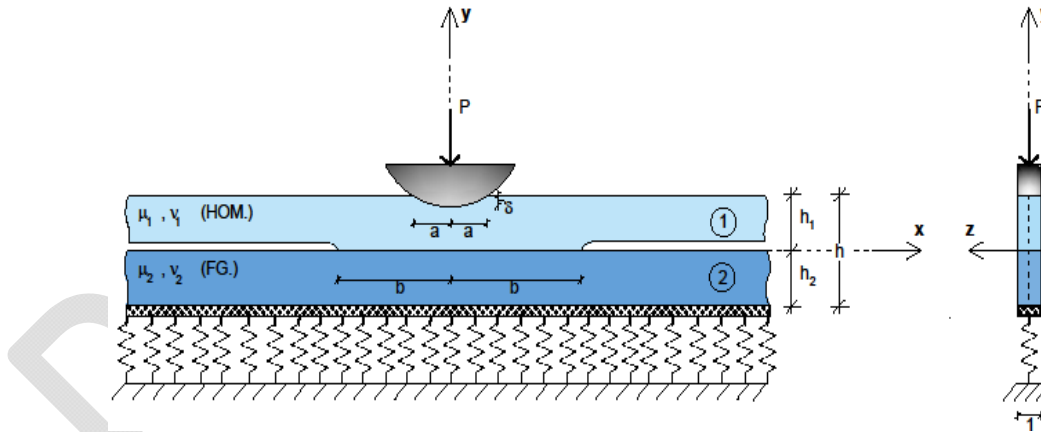
Fig. 1 - Geometry and loading of contact problem.
