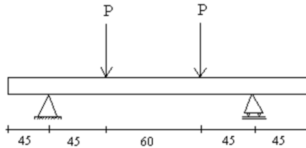
Figure 1 - Four-point loading configuration of a sleeper (dimensions are in cm).
