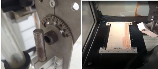
Figure 5. Adjustment unit for blasting angles and its use.
