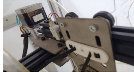
Figure 6. Stepper motors and drive system
