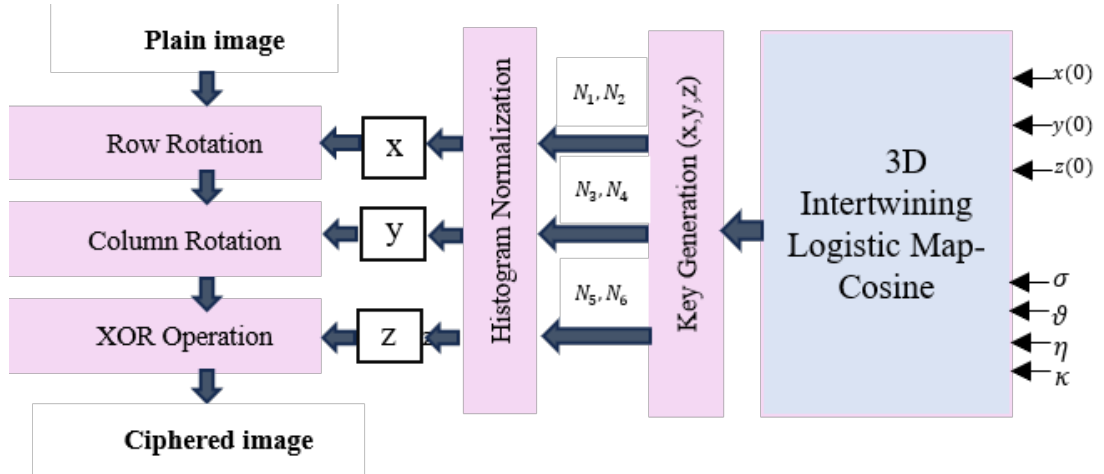
Fig. 1: Encryption steps based on 3D Intertwining LM-Cosine.
