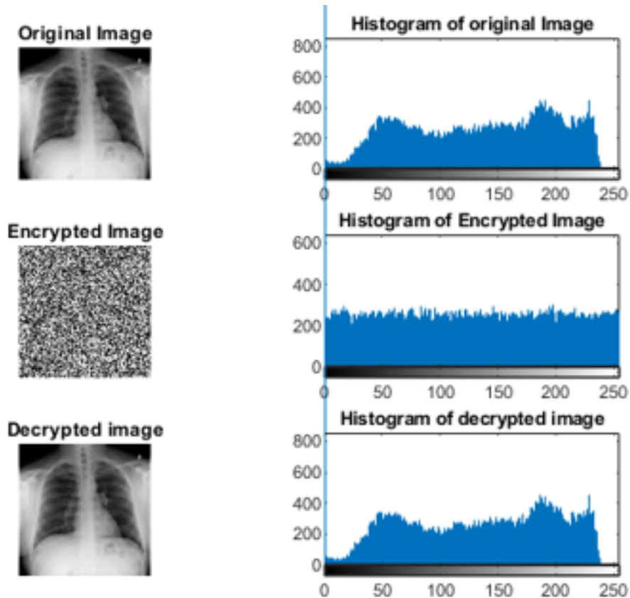
Fig. 3: Histogram plot results of plain, encrypted, and decrypted M3 images.
