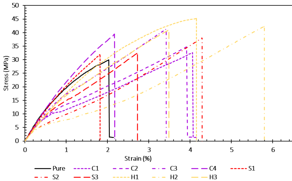
Figure 3. Engineering stress-strain curves of nanocomposites
