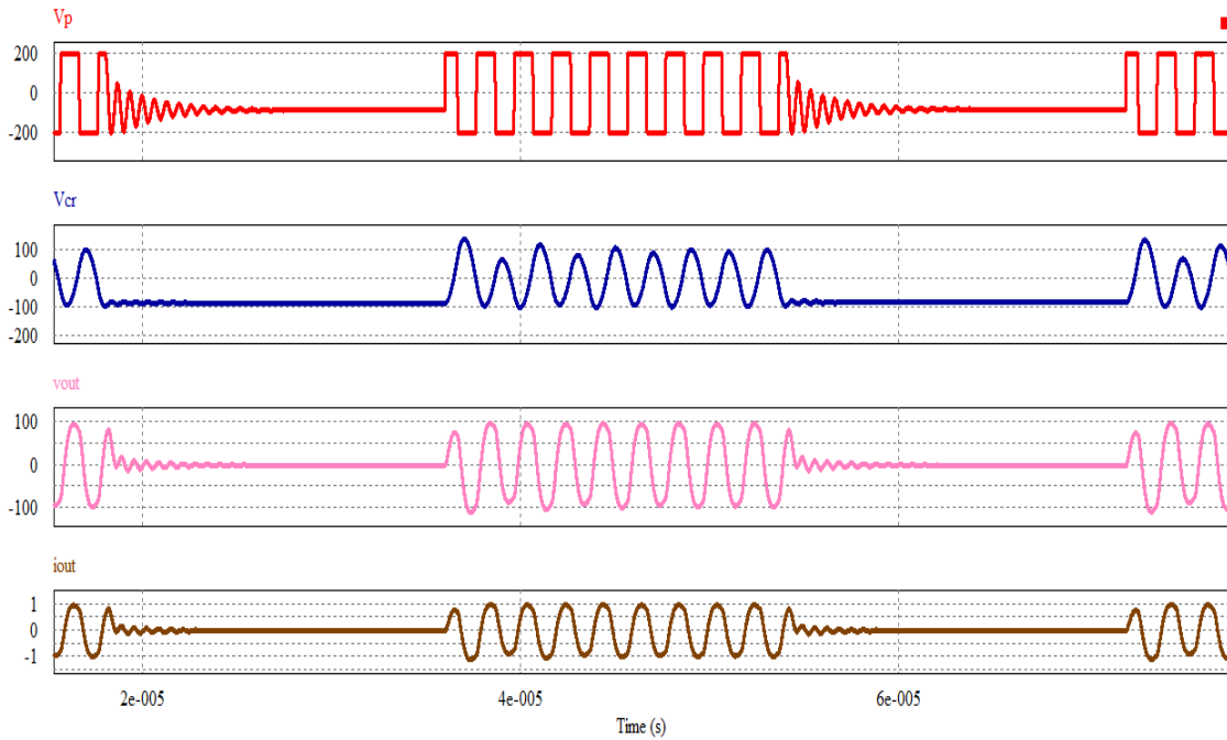
Figure 8. Waveforms for blend mode. Primary voltage V_p , resonant capacitor voltage V_{cr} , output voltage v_{out} , and output current i_{out}
