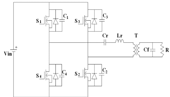
Figure 2. The full-bridge class DE resonant inverter.
