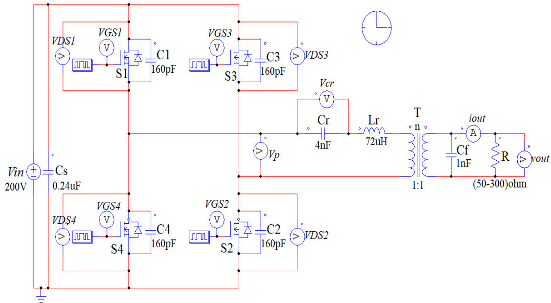
Figure 5. The simulated circuit of the proposed inverter
