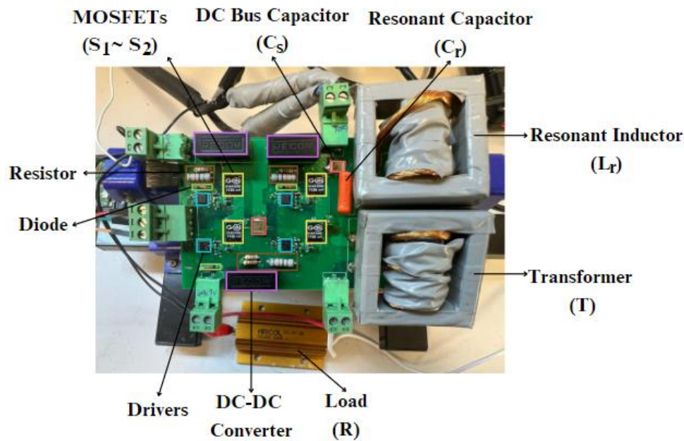
Figure. Prototype design built in the laboratory
