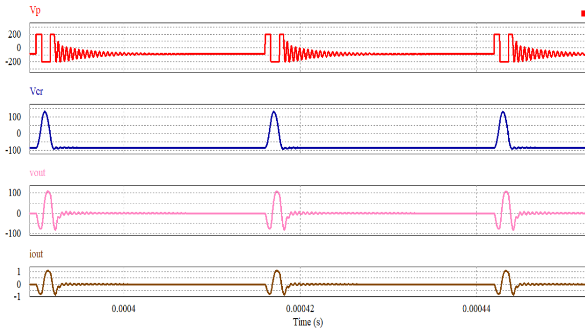
Figure 9. Waveforms for coagulation mode. Primary voltage V_p , resonant capacitor voltage V_{cr} , output voltage v_{out} , and output current i_{out}
