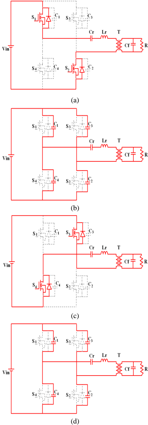
Figure 3. Operating states of full-bridge class DE resonant inverter. (a) [t 0 , t 1 ], (b) [t 1 , t 2 ], (c) [t 2 , t 3 ], (d) [t 3 , t 4 ]
