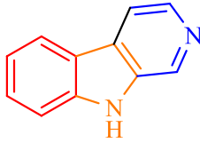
Figure 1. Chemical structure of norharmane.
