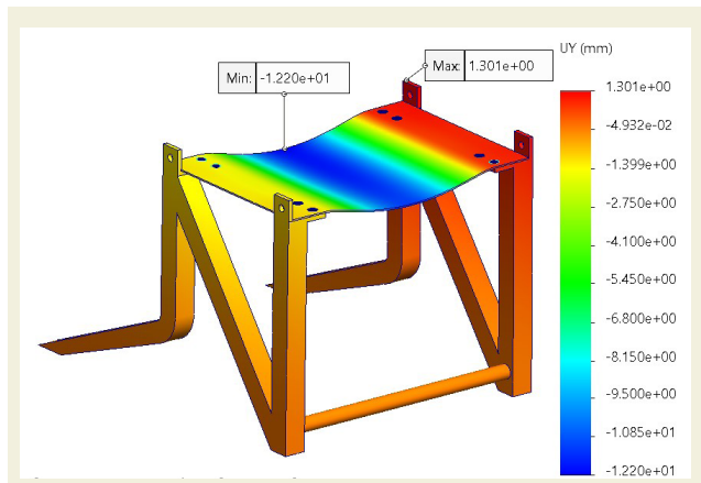
Figure 27. Y-Component of Displacement (simulation 4).
