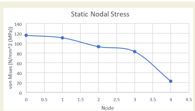
Figure 13. Static nodal stress (simulation 1)
