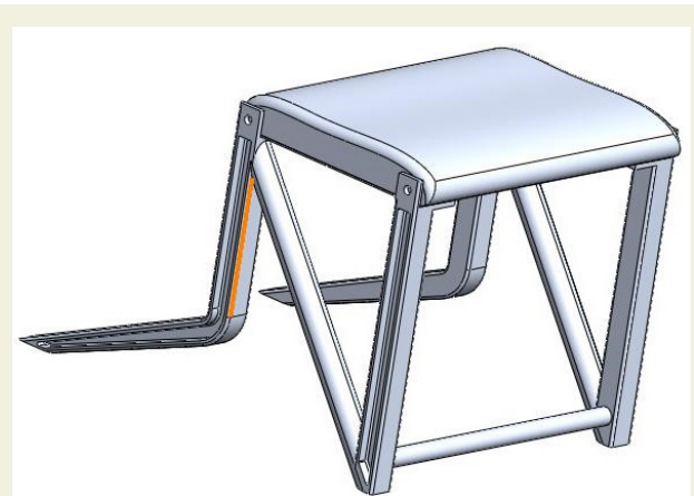
Figure 34. Fully Assembled Optimized Seat Frame (for simulation 1-AL7075-T6(SN)).
