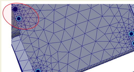
Figure 9. Connection pins prescribed in SOLIDWORKS.
