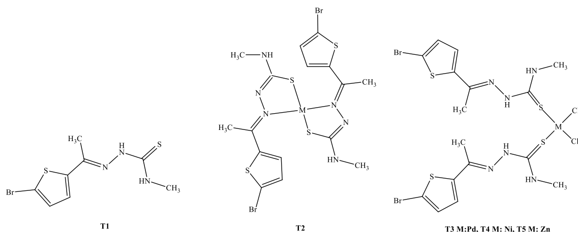
Figure 2. Compounds synthesized by Çakmakçı et al. [17]
