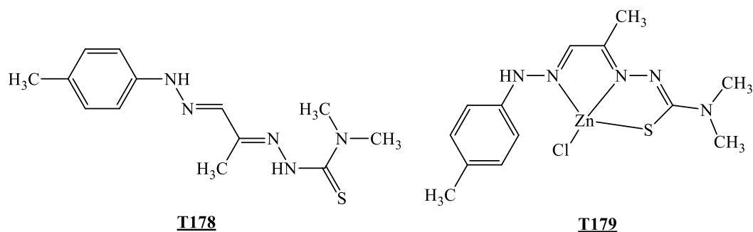
Figure 25. The compounds synthesized by Aljahdali et al. [40]
