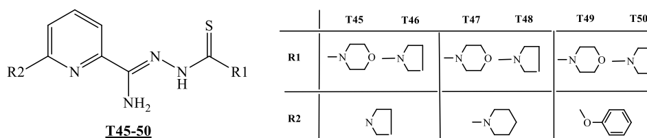
Figure 7. Thiosemicarbazone derivatives synthesized by Ziembicka [22]
