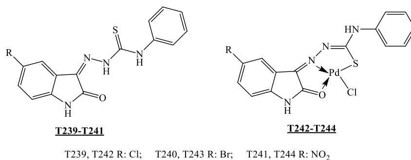
Figure 31. The compounds synthesized by Munikumari et al.
