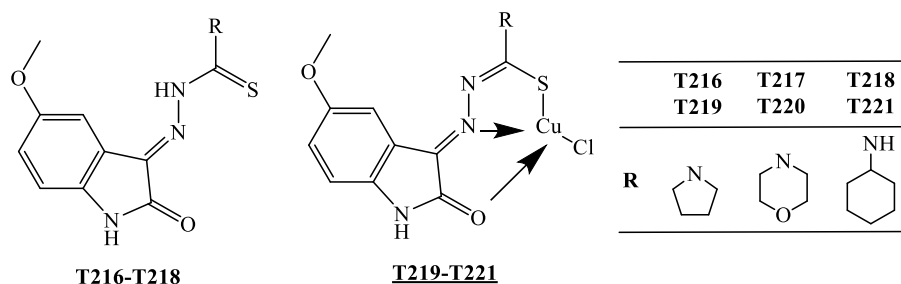
Figure 29. The compounds synthesized by Aneesrahman et al. [44]
