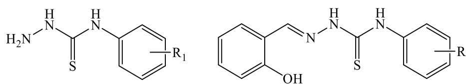
Figure 24. The phenylthiosemicarbazones synthesized by Ameryckx et al. [39]
