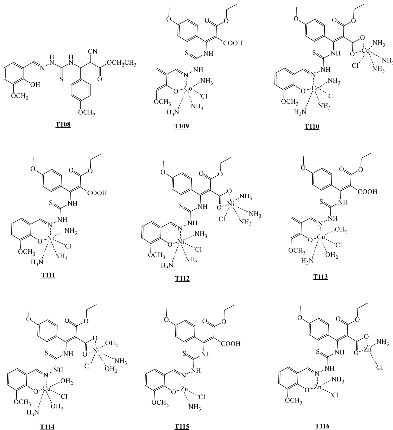
Figure 17. The compounds synthesized by Gaber et al. [32]
