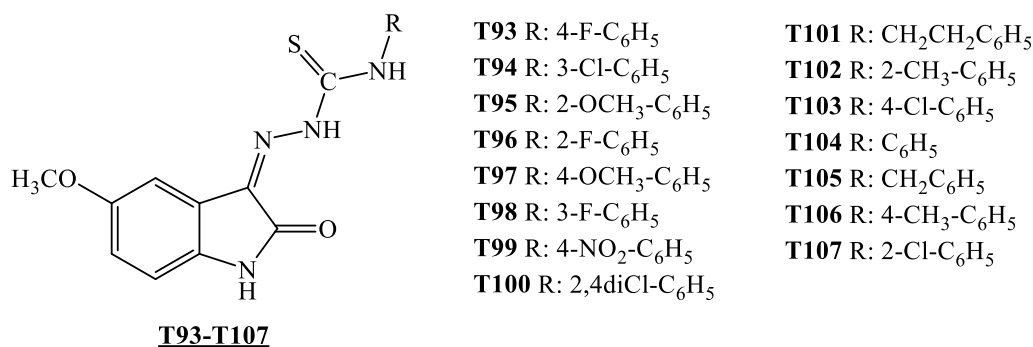
Figure 16. The compounds synthesized by Koçyiğit et al.[31]
