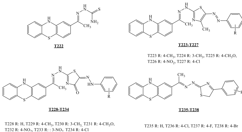
Figure 30. The compounds synthesized by Alsharekh et al. [45]
