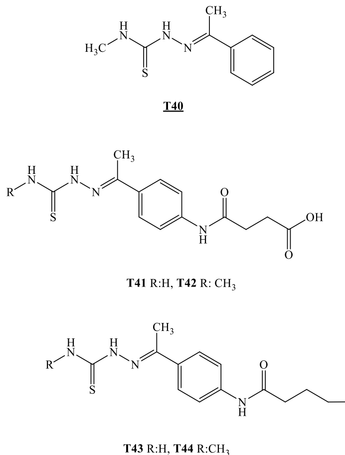
Figure 6. Thiosemicarbazone ligands synthesized by Beltr'an-Torres [21]
