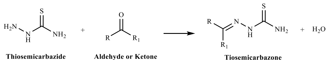
Figure 1. General structure of thiosemicarbazones [5]
