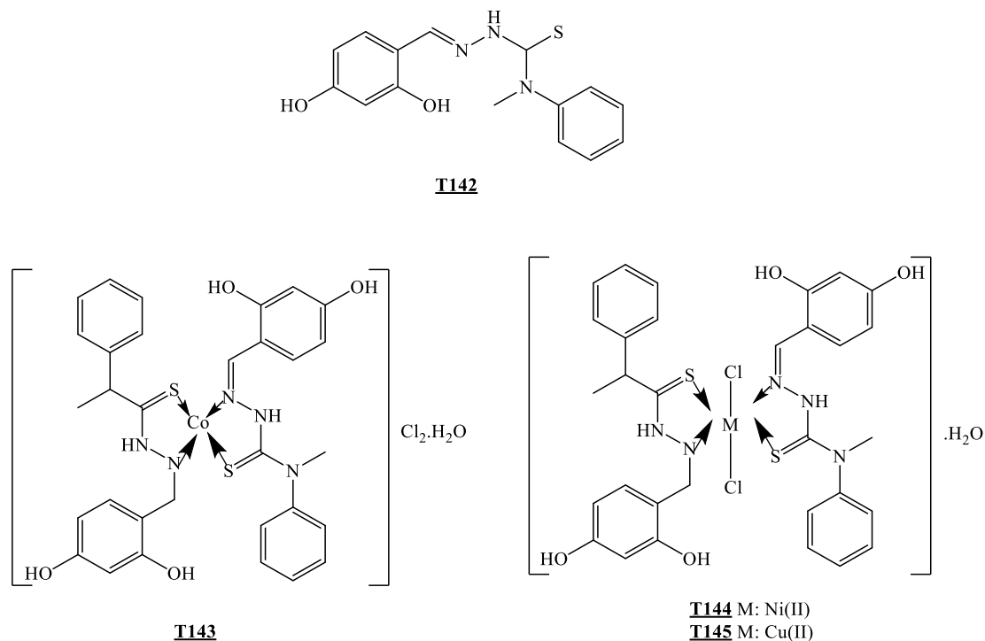
Figure 21. The compounds synthesized by Nibila et al. [36]
