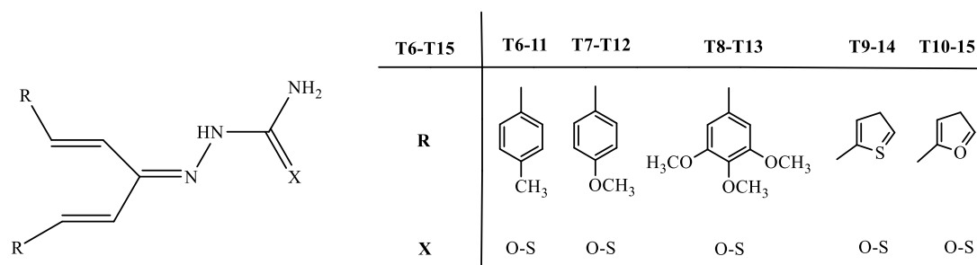
Figure 3. Compounds synthesized by Sharma et al. [18]
