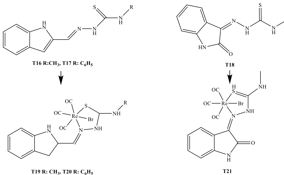
Figure 4. Compounds synthesized by Diksha et al. [19]
