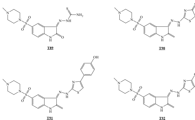
Figure 15. The compounds synthesized by Alzaharani et al. [30]
