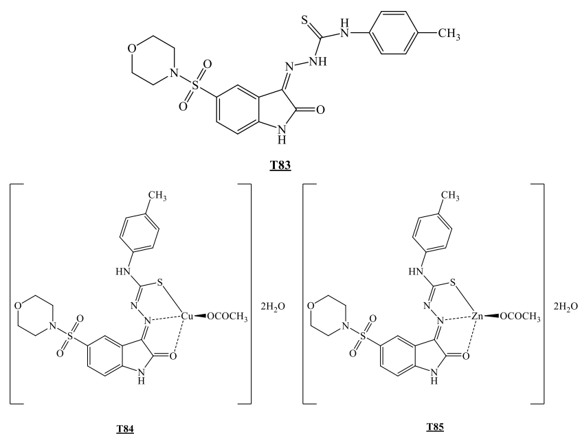
Figure 13. The compounds synthesized by Ragap et al. [28]
