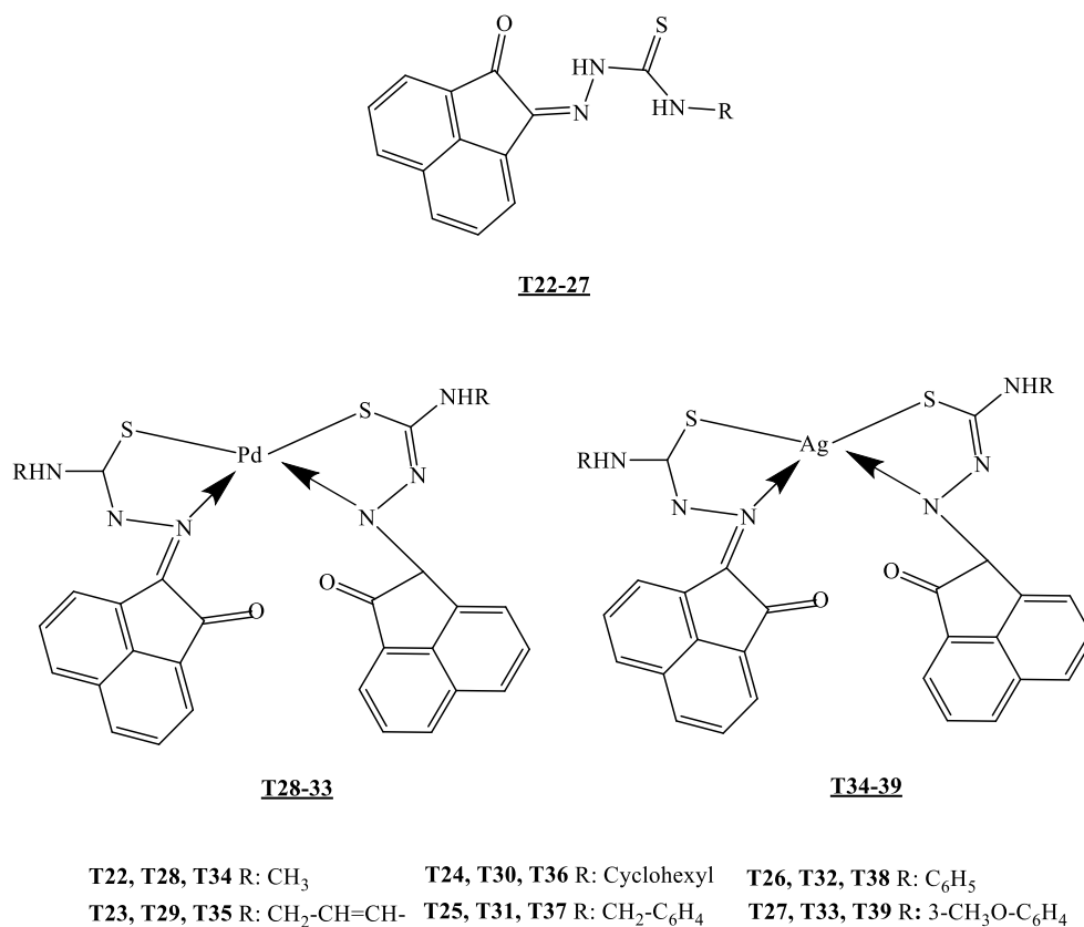
Figure 5. Thiosemicarbazone derivatives synthesized by Aly et al.[20]
