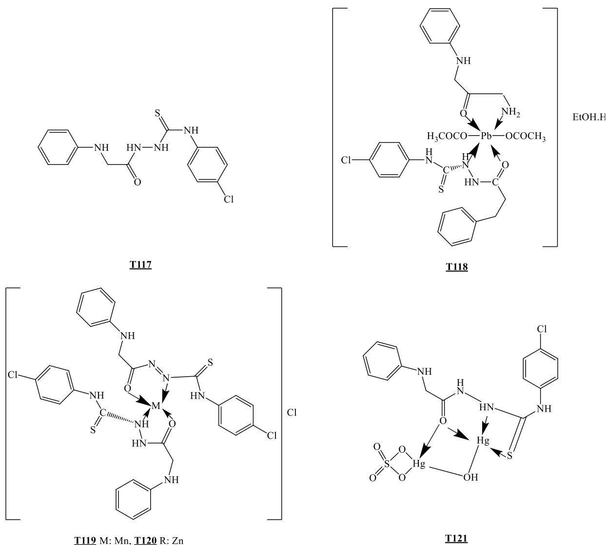
Figure 18. The thiosemicarbazones and their complexes synthesized by Alzahrani et al. [33]
