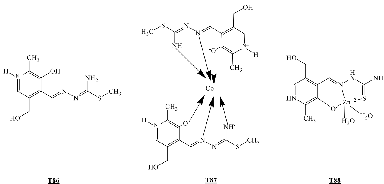
Figure 14. Compounds that Jevtovic et al. investigated for their antimicrobial activities [29]
