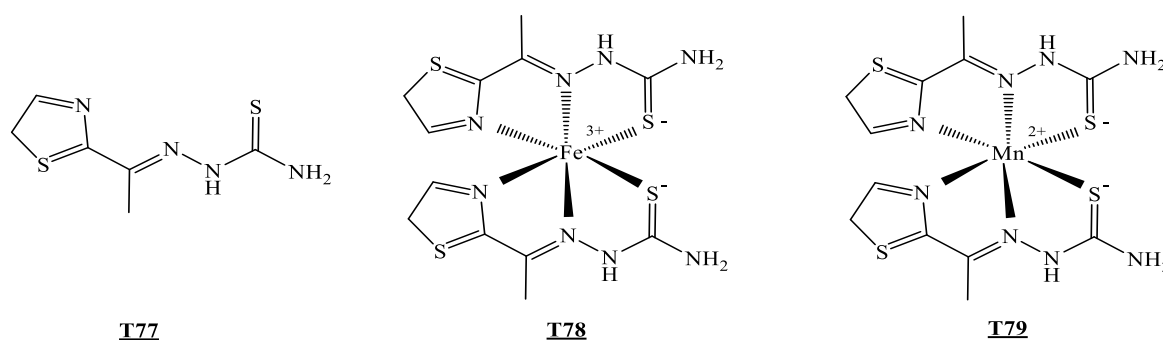
Figure 11. The compounds synthesized by Stojickov et al. [26]
