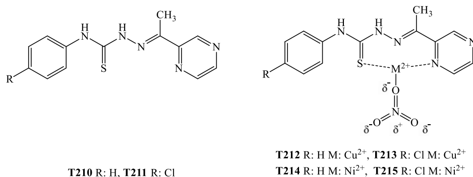
Figure 28. Thiosemicarbazone complexes synthesized by Pole-Ceron [43]
