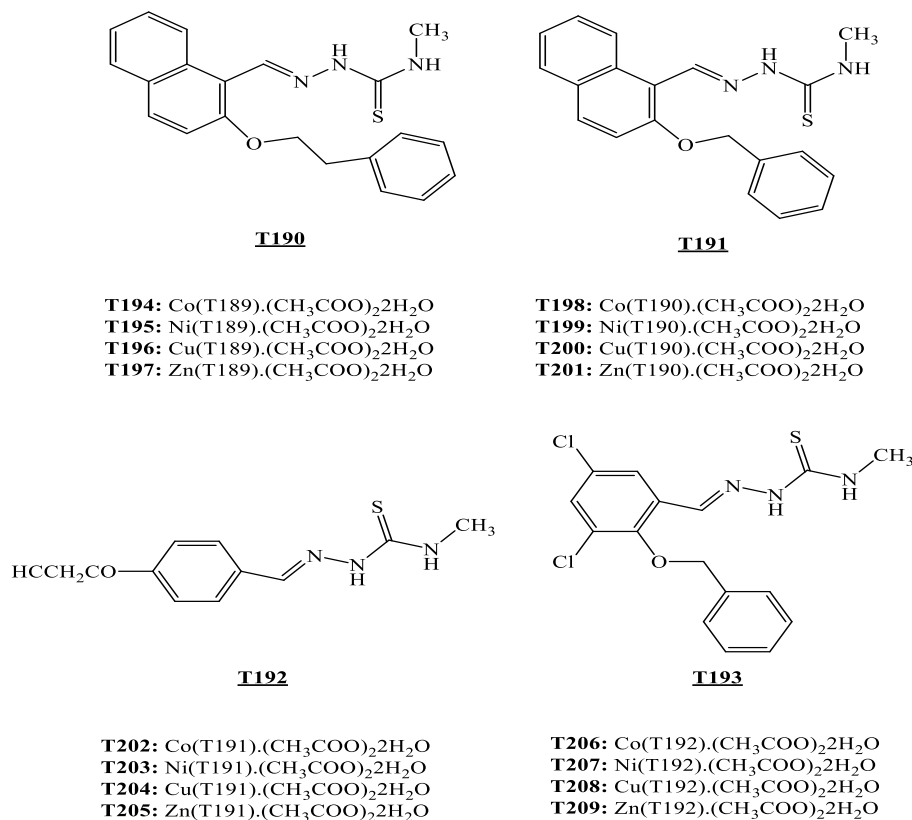
Figure 27. The compounds synthesized by Devi et al. [42]
