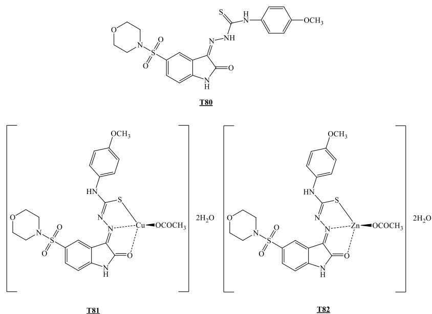
Figure 12. The compounds synthesized by Ezzet et al. [27]
