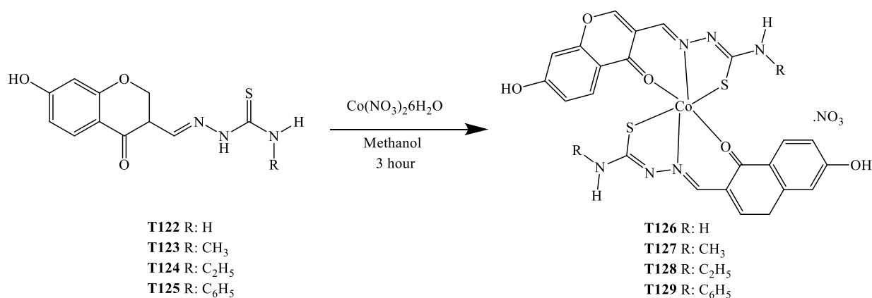
Figure 19. The compounds synthesized by Kalaiarasi et al. [34]
