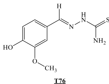
Figure 10. Thiosemicarbazone derivative synthesized by Swaminathan [25]
