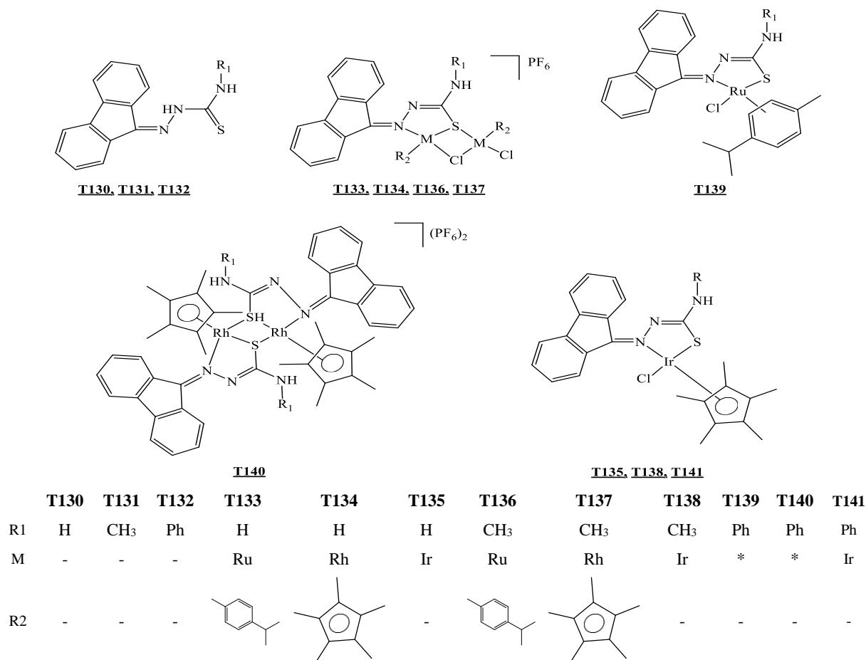
Figure 20. The compounds synthesized by Nongpiur et al. [35].
