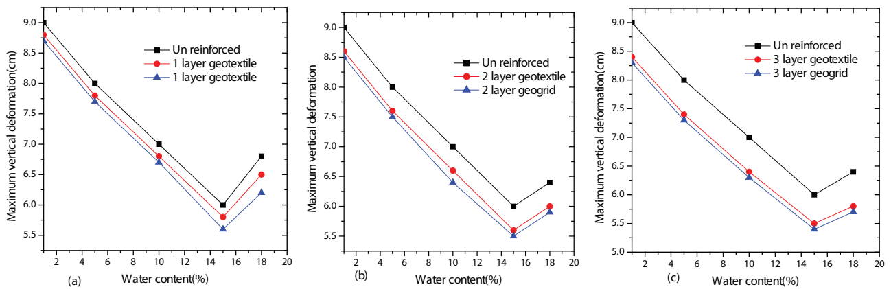
Figure 6. Effect of vertical deformation at moisture content. (a) Single layer reinforcement. (b) Two layer reinforcement. (c) Three layer reinforcement
