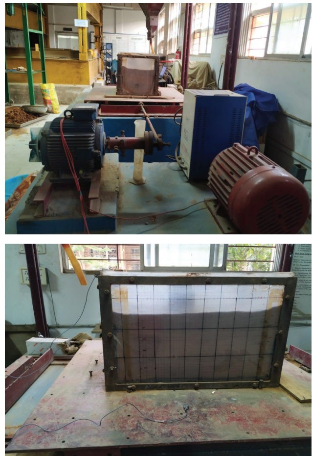
Figure 5. Construction process of model foundation (a) Shake Table set up (b) accelerometer connected at top and bottom of shake table.
