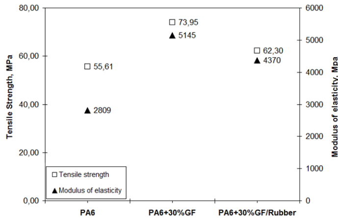
Figure 2. Tensile strength and modulus values of PA6 and PA6 composites
