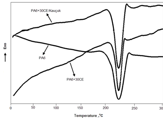
Figure 5. DSC thermogram of PA6 and composites
