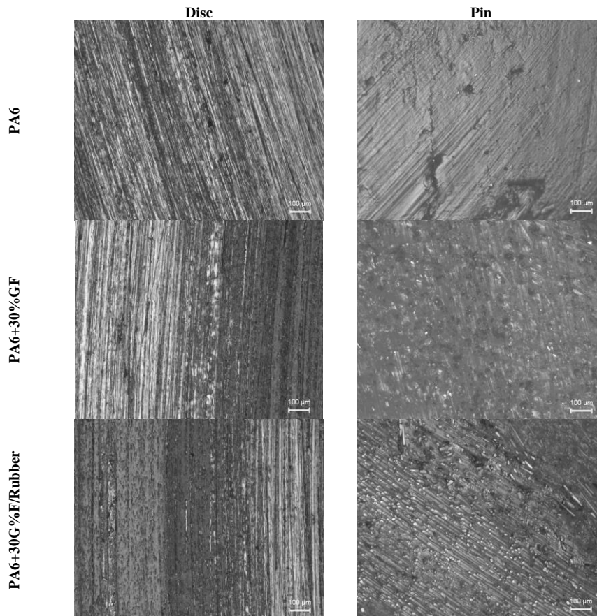
Figure 11. Wear surface images of PA6 and composites
