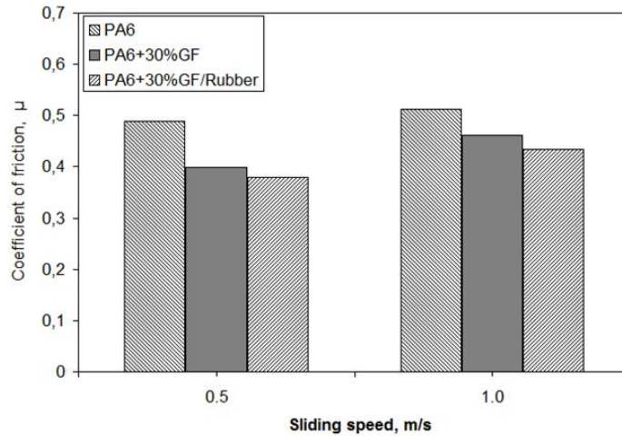
Figure 8. Relation of friction coefficient-sliding speed for PA6 polymer and PA6 composites
