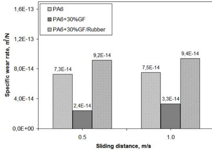
Figure 10. Relation of wear rate-sliding speed of PA6 polymer and PA6 composites
