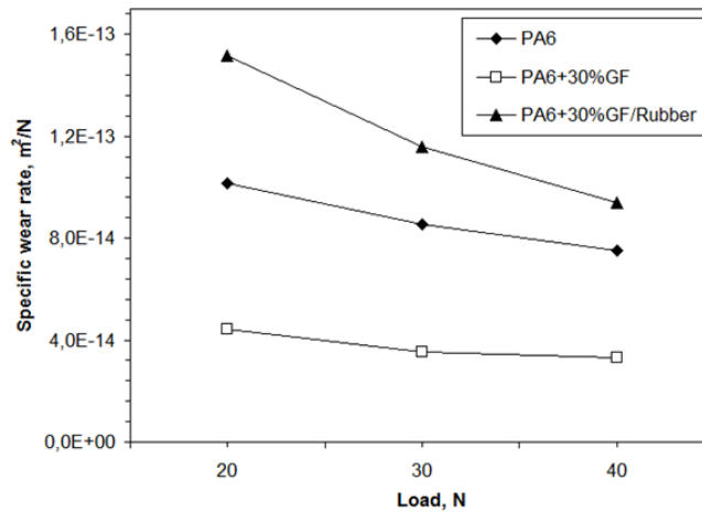
Figure 9. Relation of wear rate-applied load of PA6 polymer and PA6 composites
