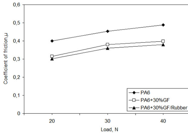
Figure 7. Relation of friction coefficient-applied load for PA6 polymer and PA6 composites
