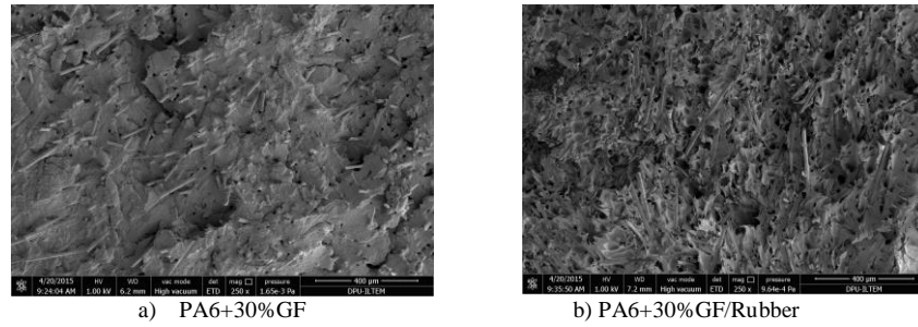
Figure 4. SEM images taken from fracture surfaces
