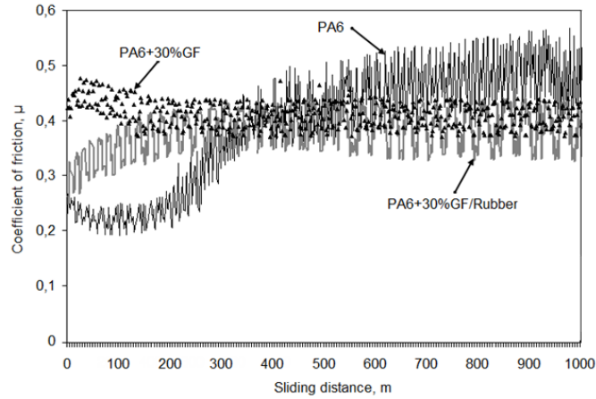
Figure 6. The coefficient of friction-sliding distance of PA6 polymer and PA6 composites (Sliding speed: 1.0 m/s, Applied load: 30 N)
