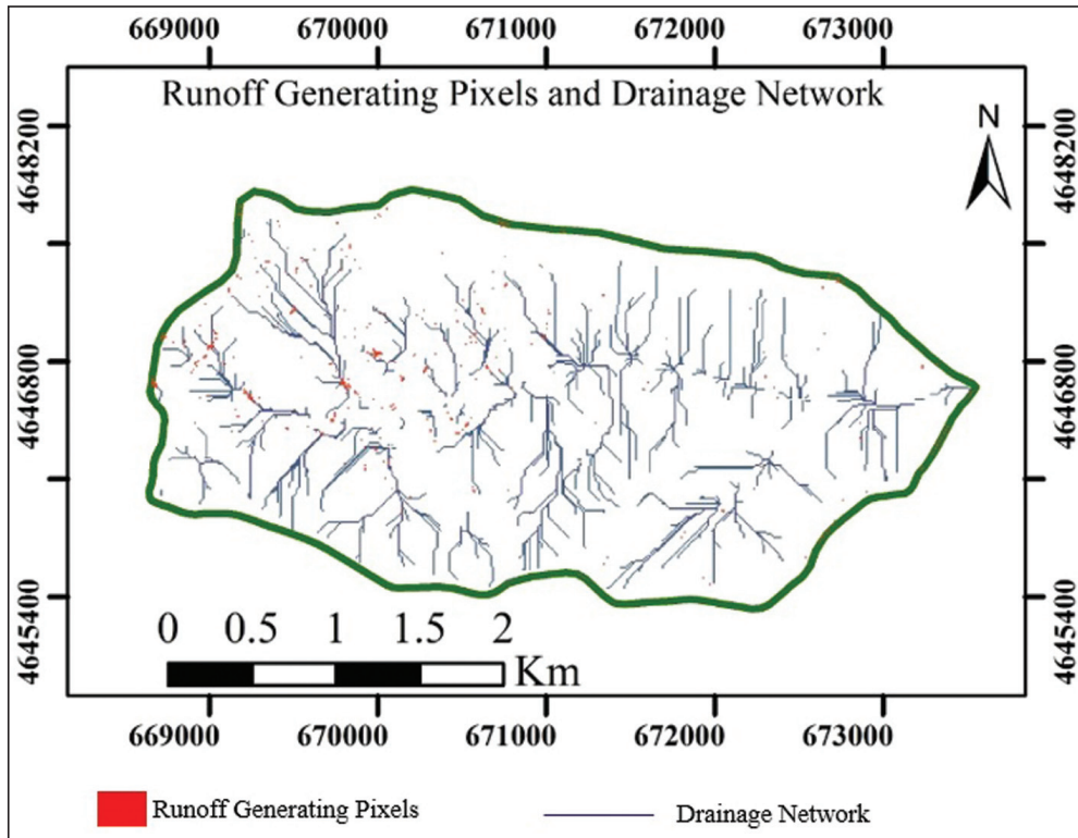
Figure 8- Potential runoff generating pixels map of June and Drainage network
