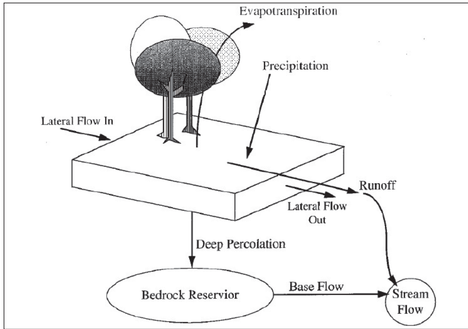
Figure 3- Hydrological processes of a cell used in SMDR model (Modified from Frankenberger et. al., 1999).
