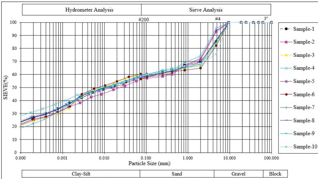
Figure 5- Grain size distributions of soil samples handled from study area.
