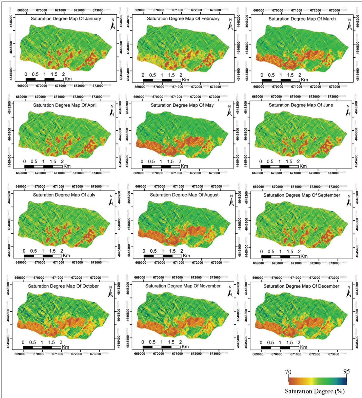
Figure 7- Monthly saturation degree variations of Demirciköy Watershed.
