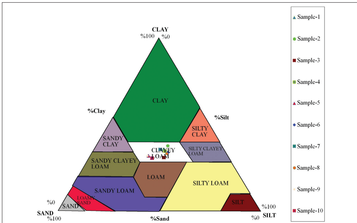
Figure 6- Textural classification of soil samples handled from the study area based on USDA soil texture classification system.
