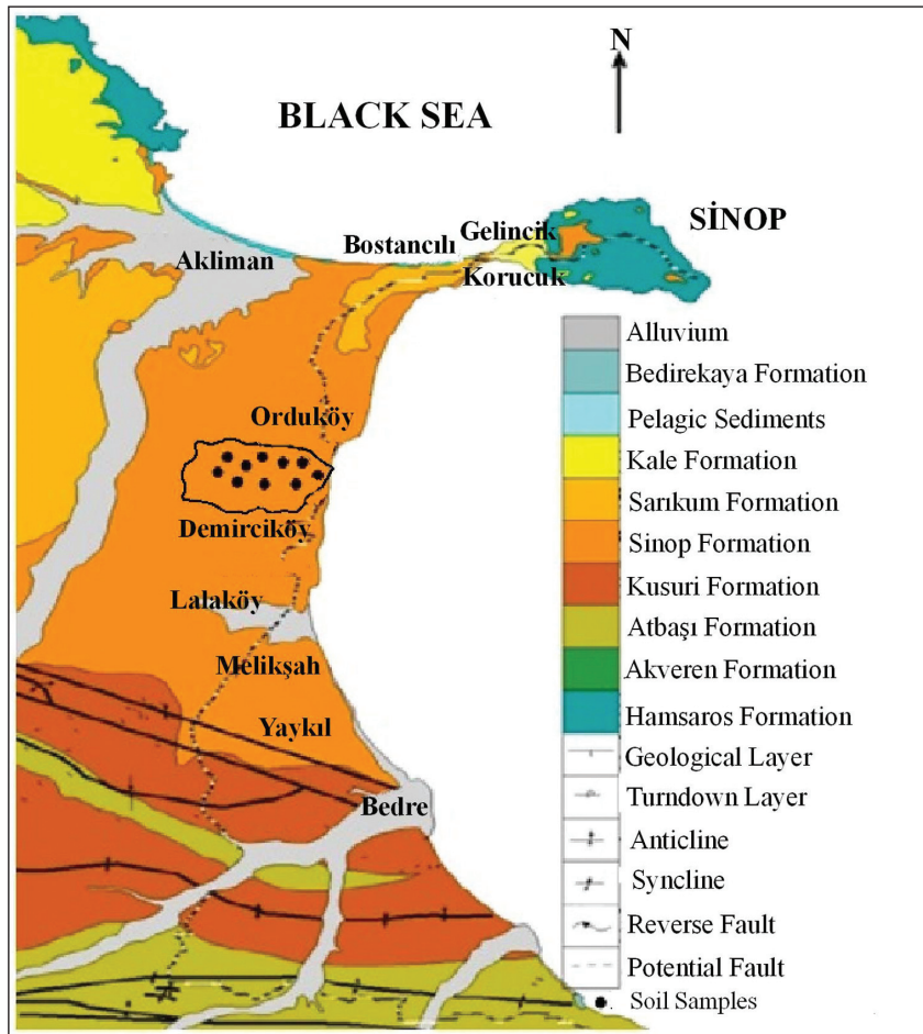
Figure 2- General geology map of the study area and its near environ (modified from Çellek, 2013).
