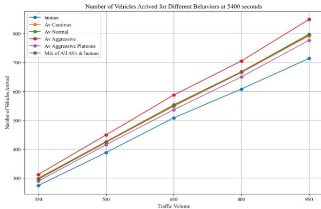
Fig. 7. Comparative arrival rates of different driving behaviors at various traffic volumes over a 5400-second simulation period
