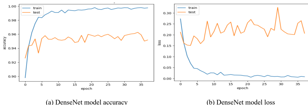
Figure 6. DenseNet model a) Model accuracy b) Model loss.
