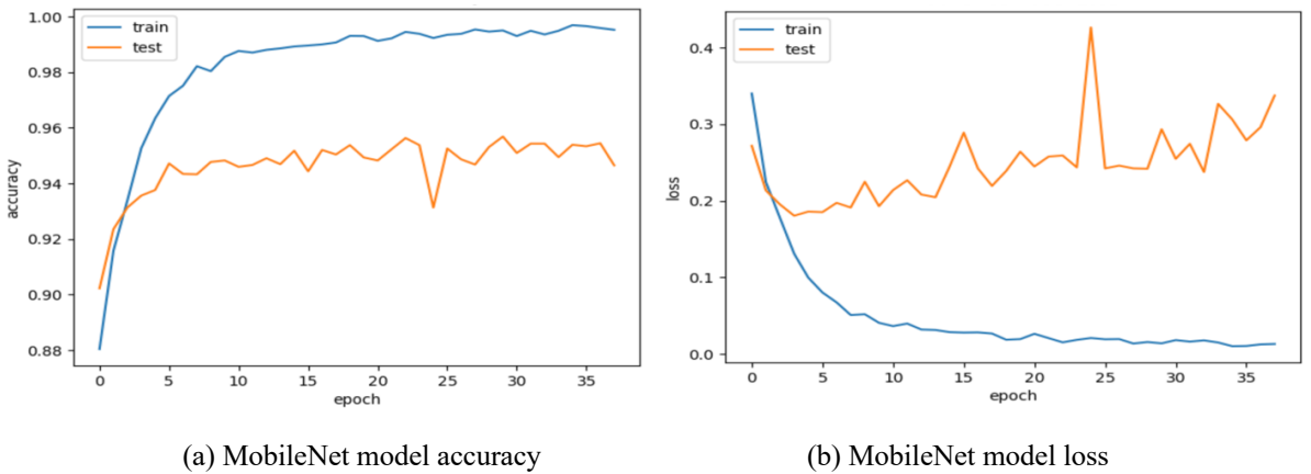
Figure 5. MobileNet model a) Model accuracy b) Model loss.
