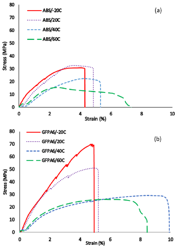
Figure 6. Stress vs strain diagram of a) ABS and b) GFPA6 [37]
