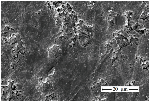
Figure 7. SEM image of non-sintered MW40 specimen.
