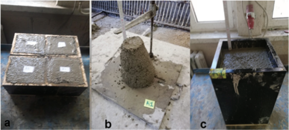
Figure 6 - Fresh Concrete Tests: a) Unit volume weight determination, b) Slump test, c) Walz test
