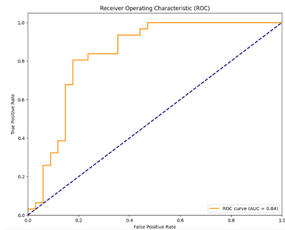
Figure 7. ROC of the ConvNextBase, which gives the best result in the histopathologic images.
