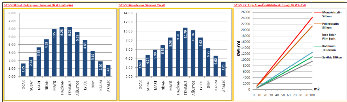
Figure 2. GEPA Ayaş daily average global solar radiation, sunshine duration and annual total energy amounts that the PV system can produce by month (Source, GEPA, 2023).
