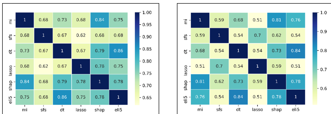
Figure 3. Jaccard index similarity of global attribute selection with 25% of threshold for; (a): Polish dataset. (b): Turkish dataset.
