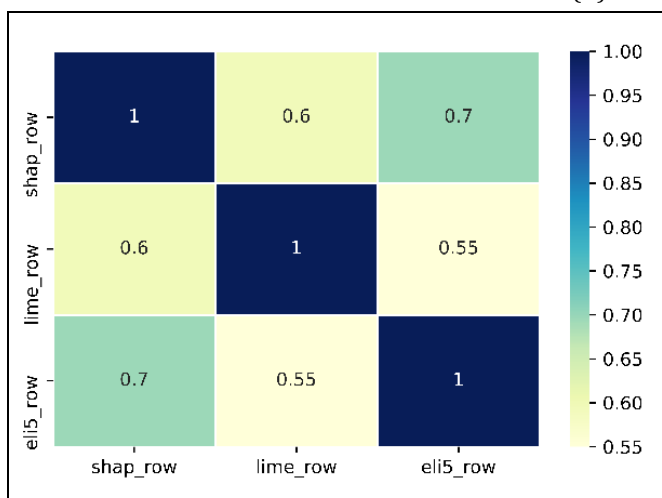
Figure 6. Jaccard index similarity of local attribute selection with 50% of threshold for; (a): Polish dataset. (b): Turkish dataset.
