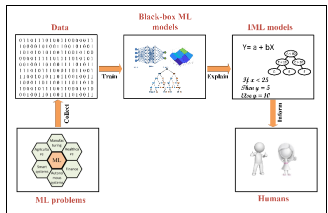
Figure 2. The general view of IML [55].
