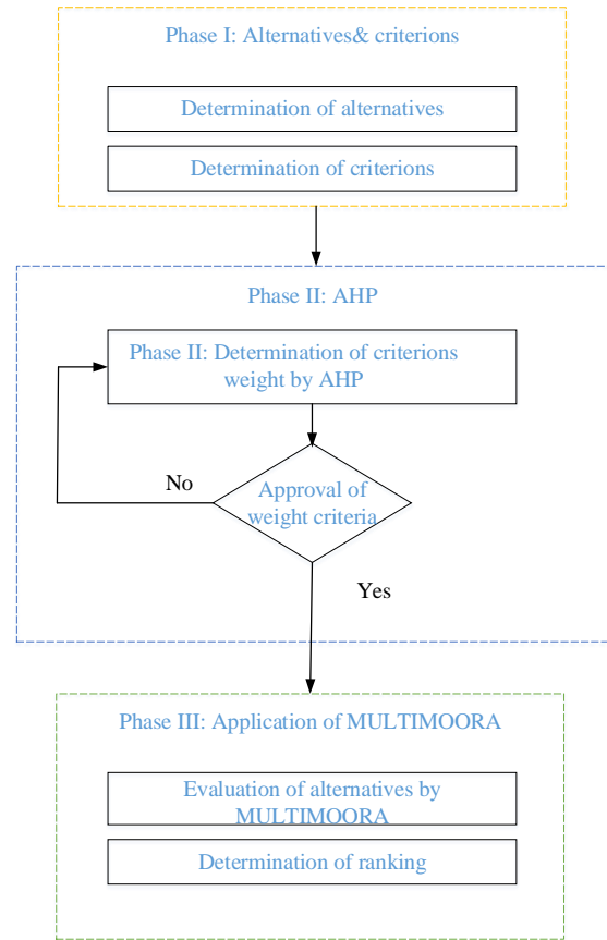
Fig. 4. Schematic representation of the MULTIMOORA method application [45]
