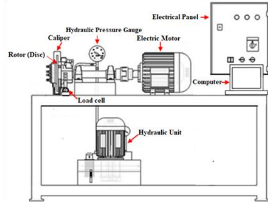
Fig. 3. Friction wear tester [48]
