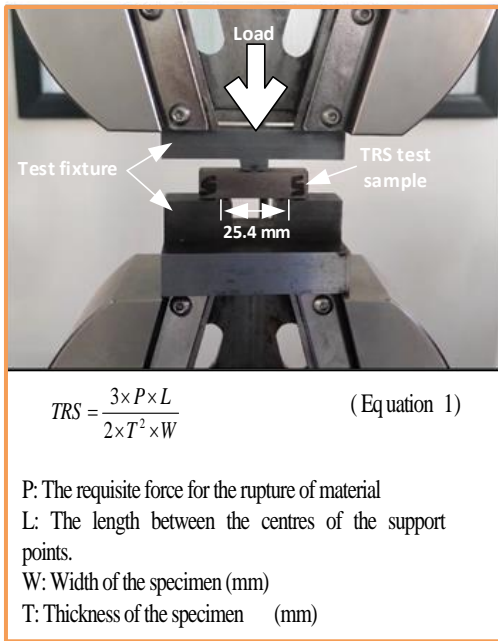
Fig. 2. TRS test set up
