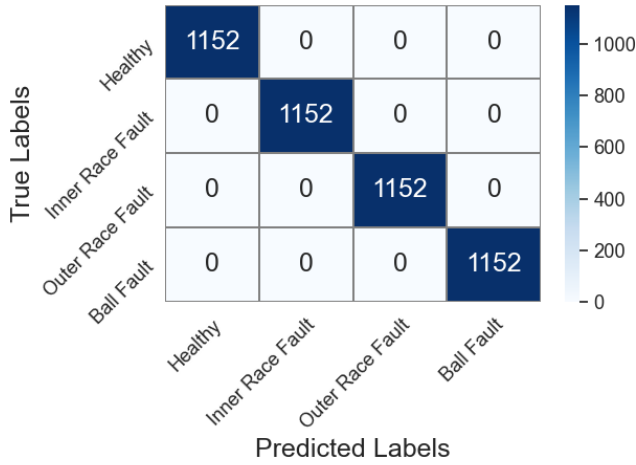
Figure 7. Confusion matrix obtained by testing the proposed LSTM-based fault classification model
