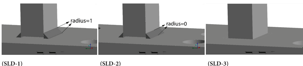
Figure 2. Welded joints FEA Modelling.
