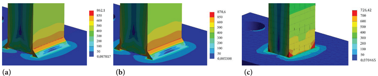
Figure 4. FEA analysis results at 186 s (a) SP1-SLD-1 (b) SP1-SLD2 (c) SP1-SLD3.
