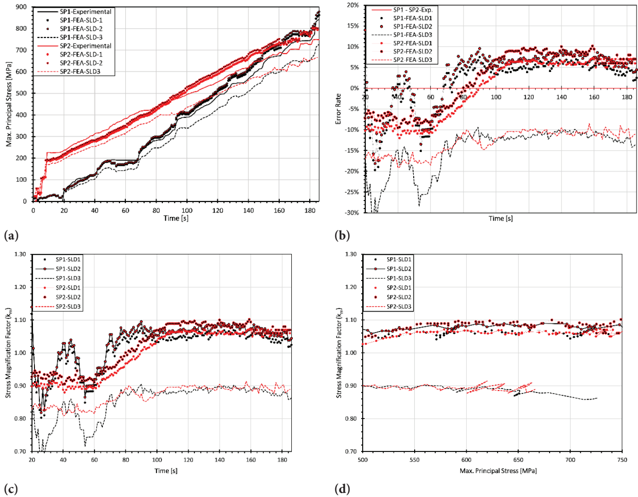
Figure 5. Comparison of experimental and numeric analysis (a) Maximum principal stress (b) Error rate (c) Stress magnification factor (d) Stress magnification factor above 500 MPa
