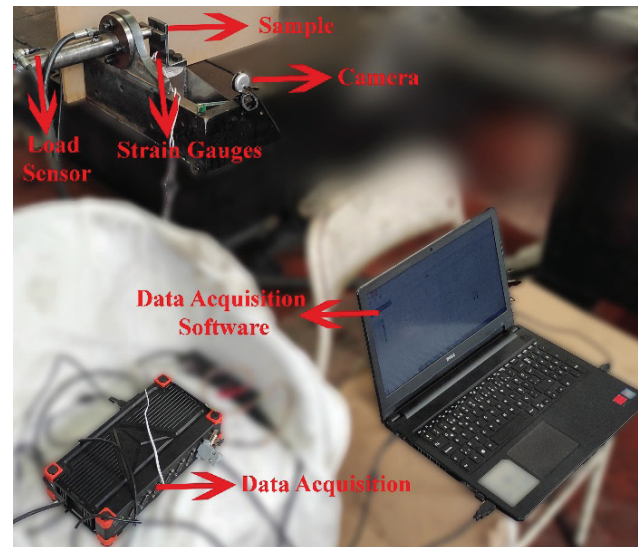
Figure 1. Experimental test setup.
