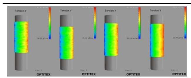
Figure 3. Tension distribution on fabric surfaces.
