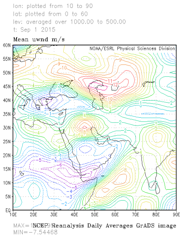
Figure 10. Zonal wind map; September 1, 2015
