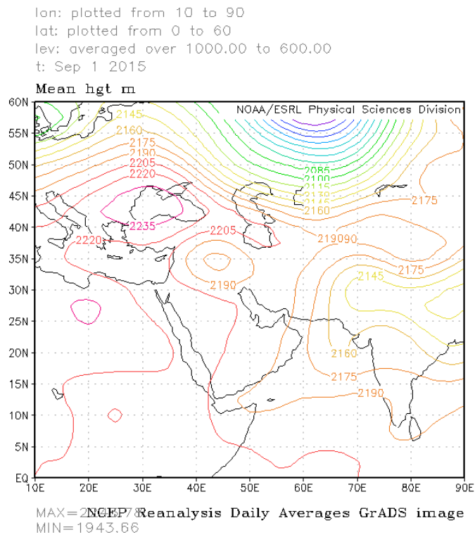
Figure 9. Geopotential height map; September 1, 2015
