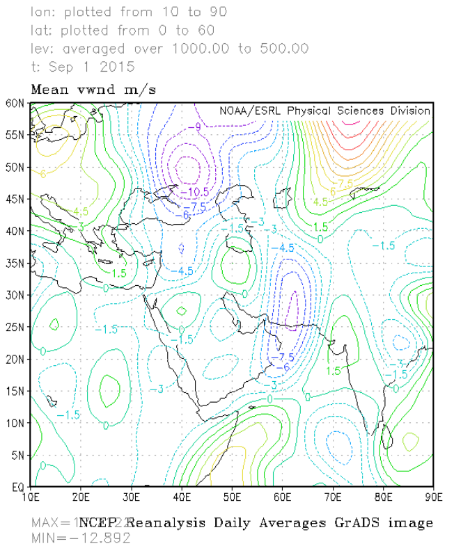
Figure 11. Meridional wind map; September 1, 2015
