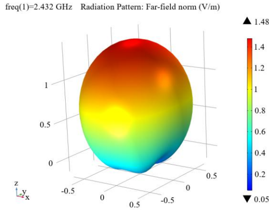
Figure 7. Simulated far-field radiation pattern of the Sierpinski carpet fractal antenna.
