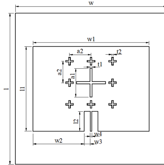
Figure 2. Dimensions of the proposed Sierpinski carpet fractal antenna.
