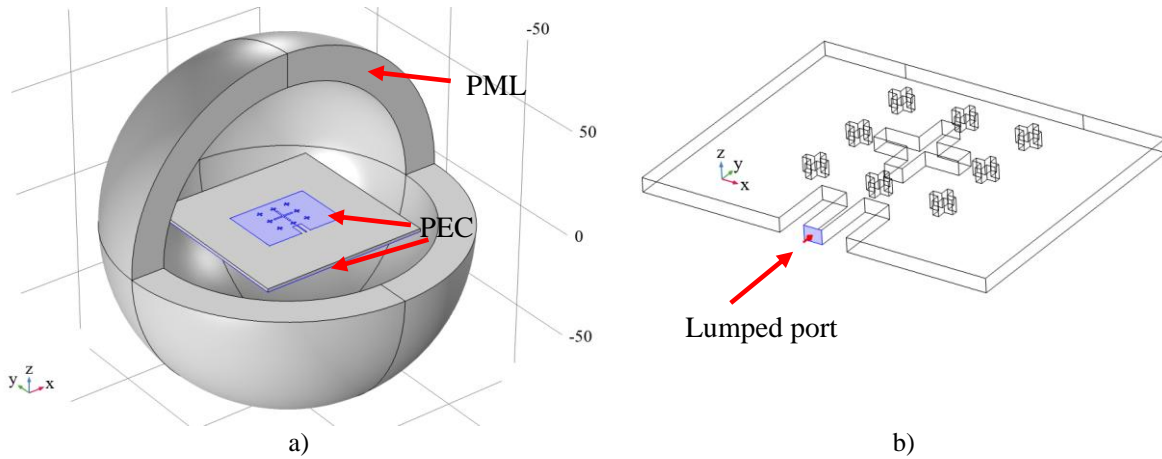
Figure 3. a) 3D view of the finite element model; b) lumped port boundary condition.
