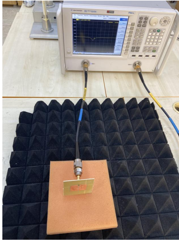
Figure 4. Measurement setup of fabricated sample.
