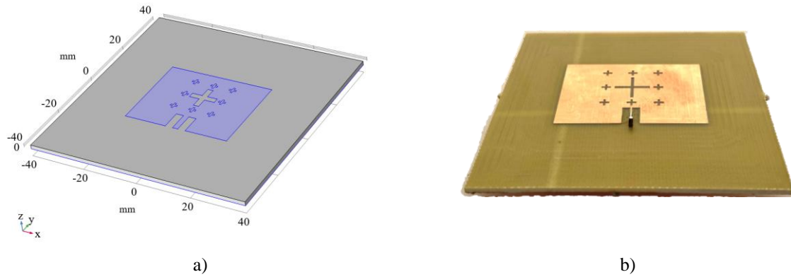
Figure 1. Structure of the Sierpinski carpet fractal patch microstrip antenna: a) Simulation model b) Fabricated sample.
