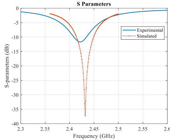
Figure 5. The simulated and experimental S-parameter (S11) response of the Sierpinski carpet fractal antenna.
