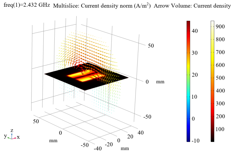
Figure 8. Current density distribution on the Sierpinski fractal antenna at the operating frequency of 2.432 GHz.
