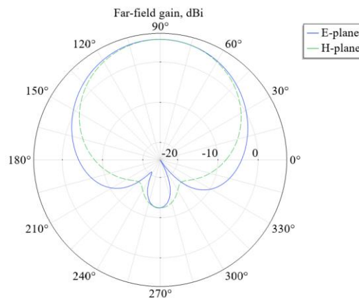
Figure 6. Simulated far-field gain pattern in dBi of the Sierpinski carpet fractal antenna.
