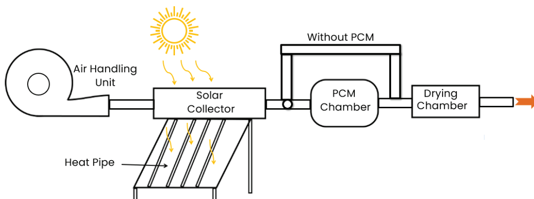
Figure 9. Forced circulation evacuated tube collector solar dryer.
