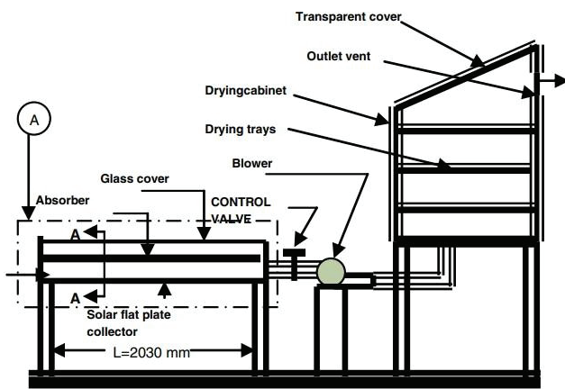
Figure 26. Schematic view of horizontally placed collector, active solar dryer operates on mixed mode [From Pardhi et al. [81], Open access].
