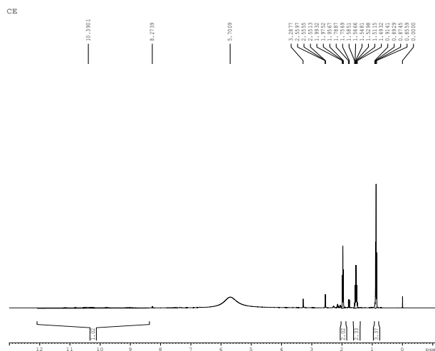
Figure 9. Proton NMR spectrum of butyhydroxamic acid.
